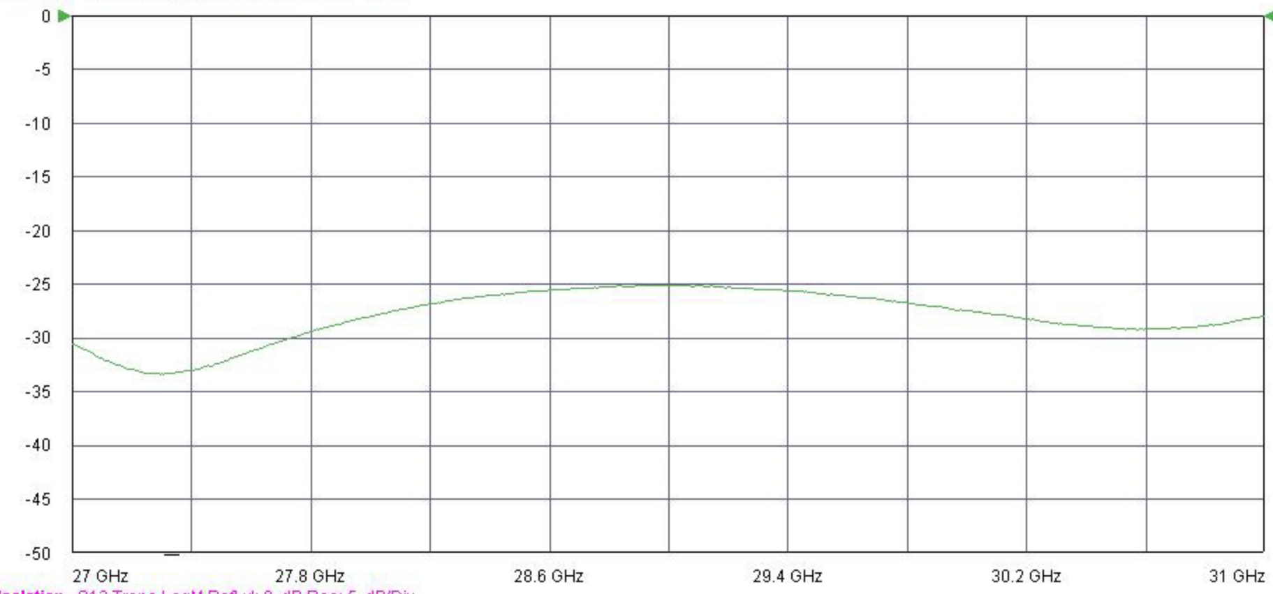
Isolation S12 Trans LogM RefLvl: 0 dB Res: 5 dB/Div
