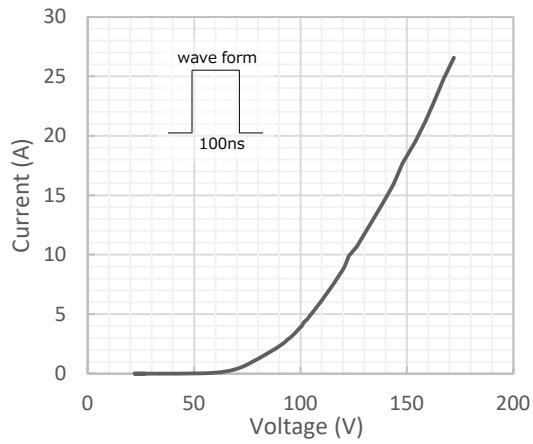
Current - Voltage (TLP)
