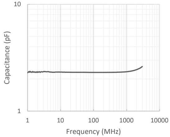
Capacitance - Freq.
