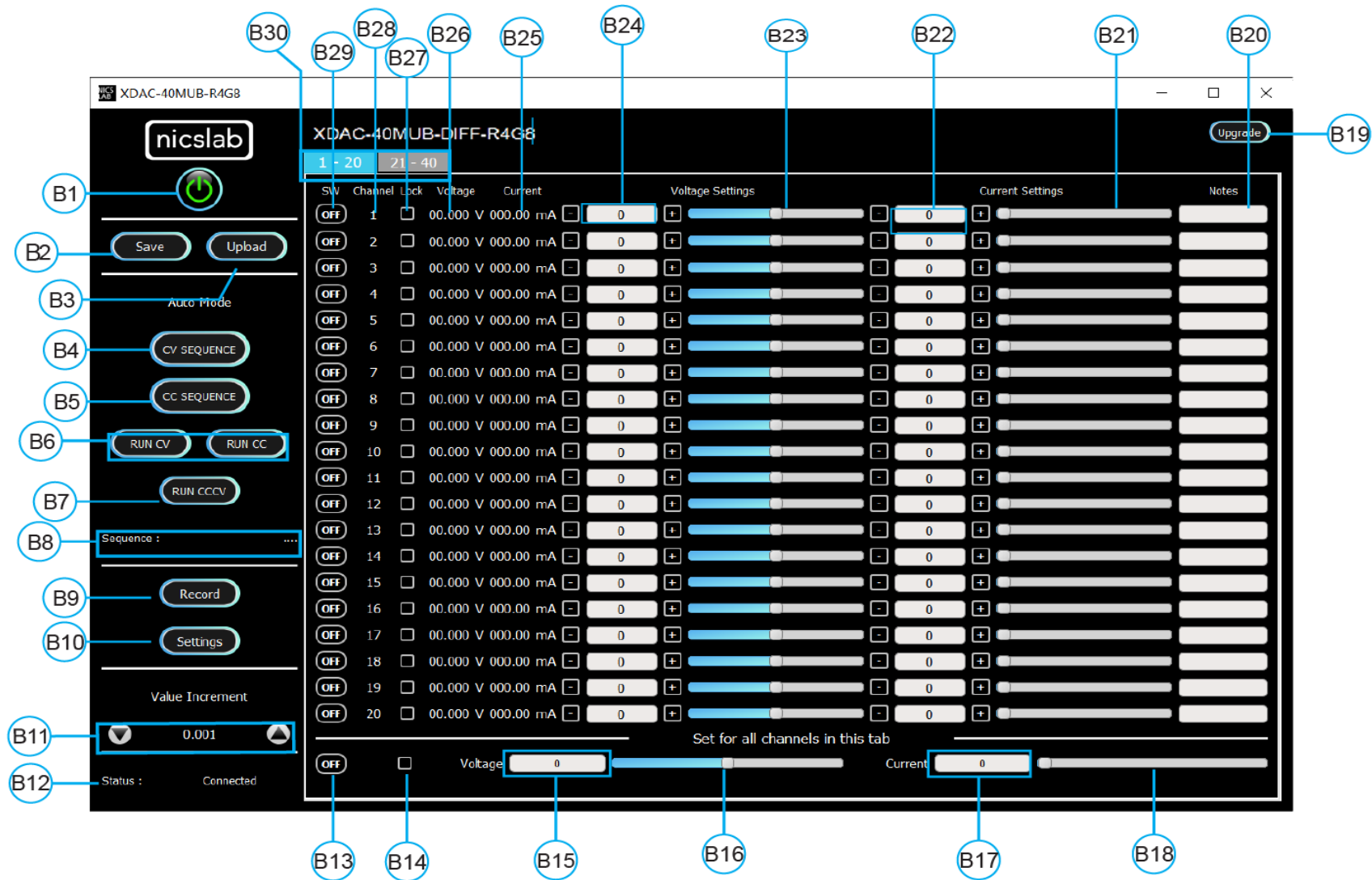
Figure 4. GUI
