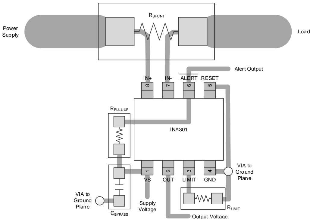
Figure 44. Recommended Layout
