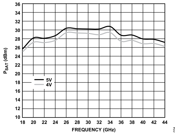
Figure 24. Saturated Output Power ( P_{SAT} ) vs. Frequency for Various Supply Voltages ( V_{DD} ), Drain Current ( I_{DQ} ) = 800 mA
