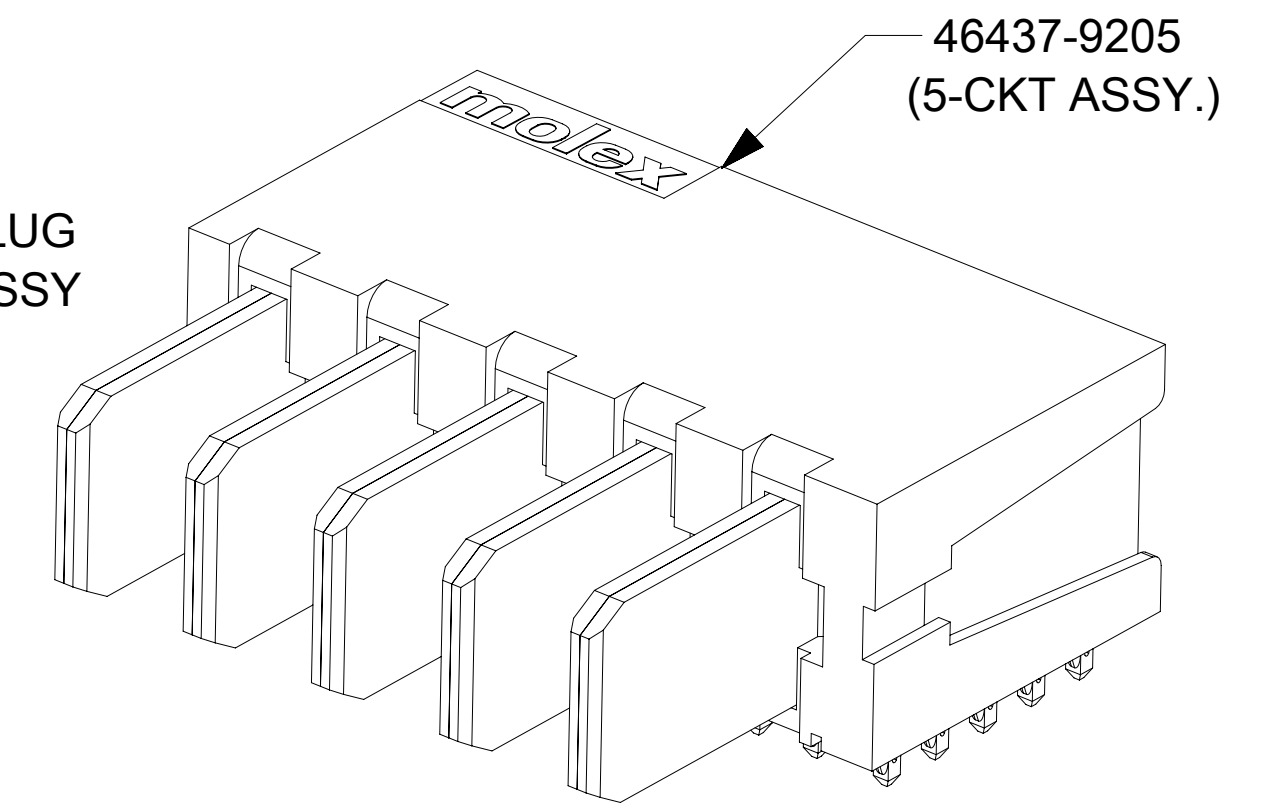
R/A PLUG ASSY. (PRESS-FIT TAIL VERSION) P/N: 46436-92** (** - 01 TO 10)
