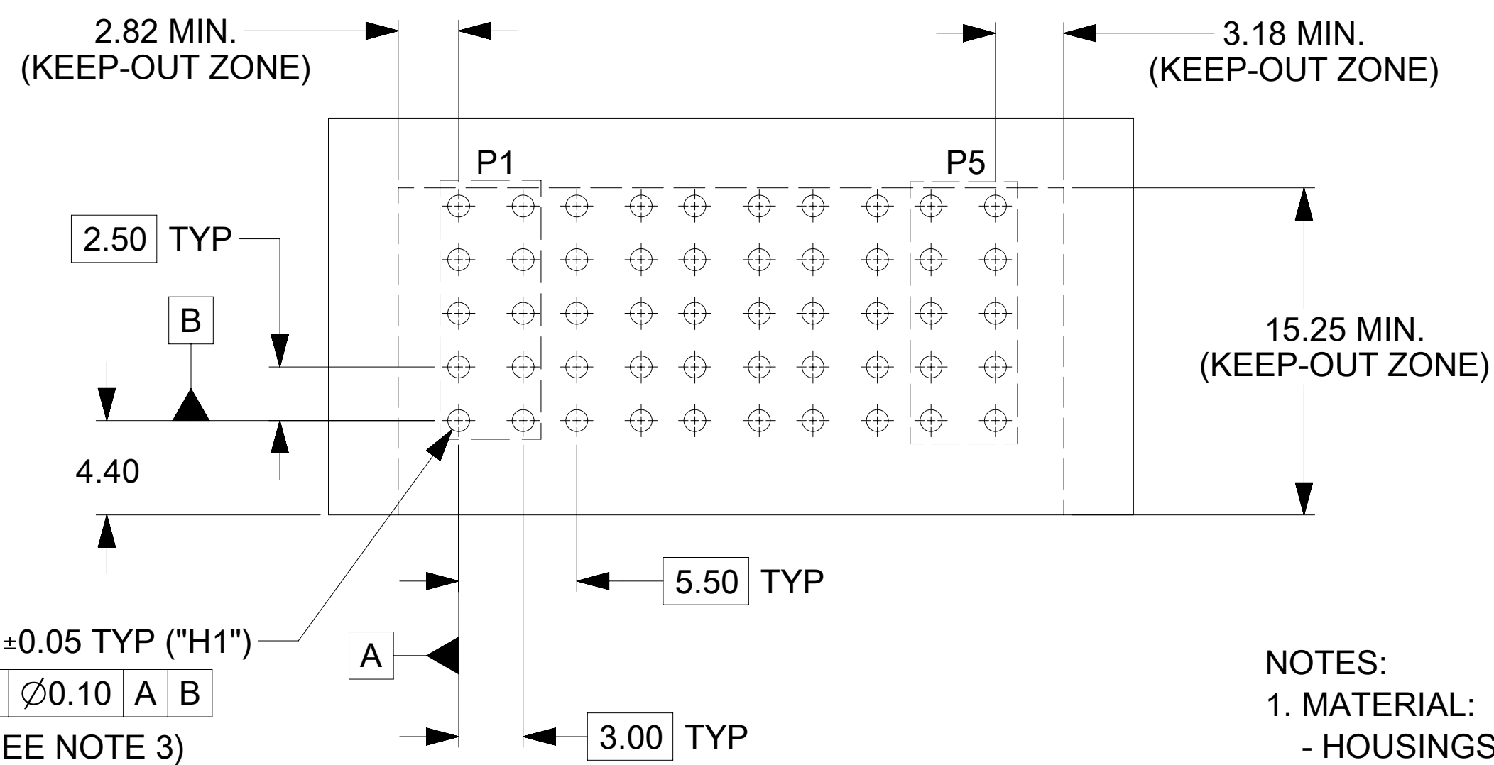
RECOMMENDED PCB LAYOUT AND KEEP-OUT ZONE
