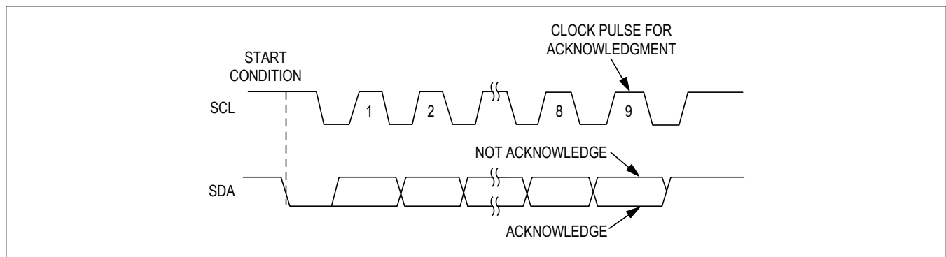
Figure 35. I 2 C Acknowledge
