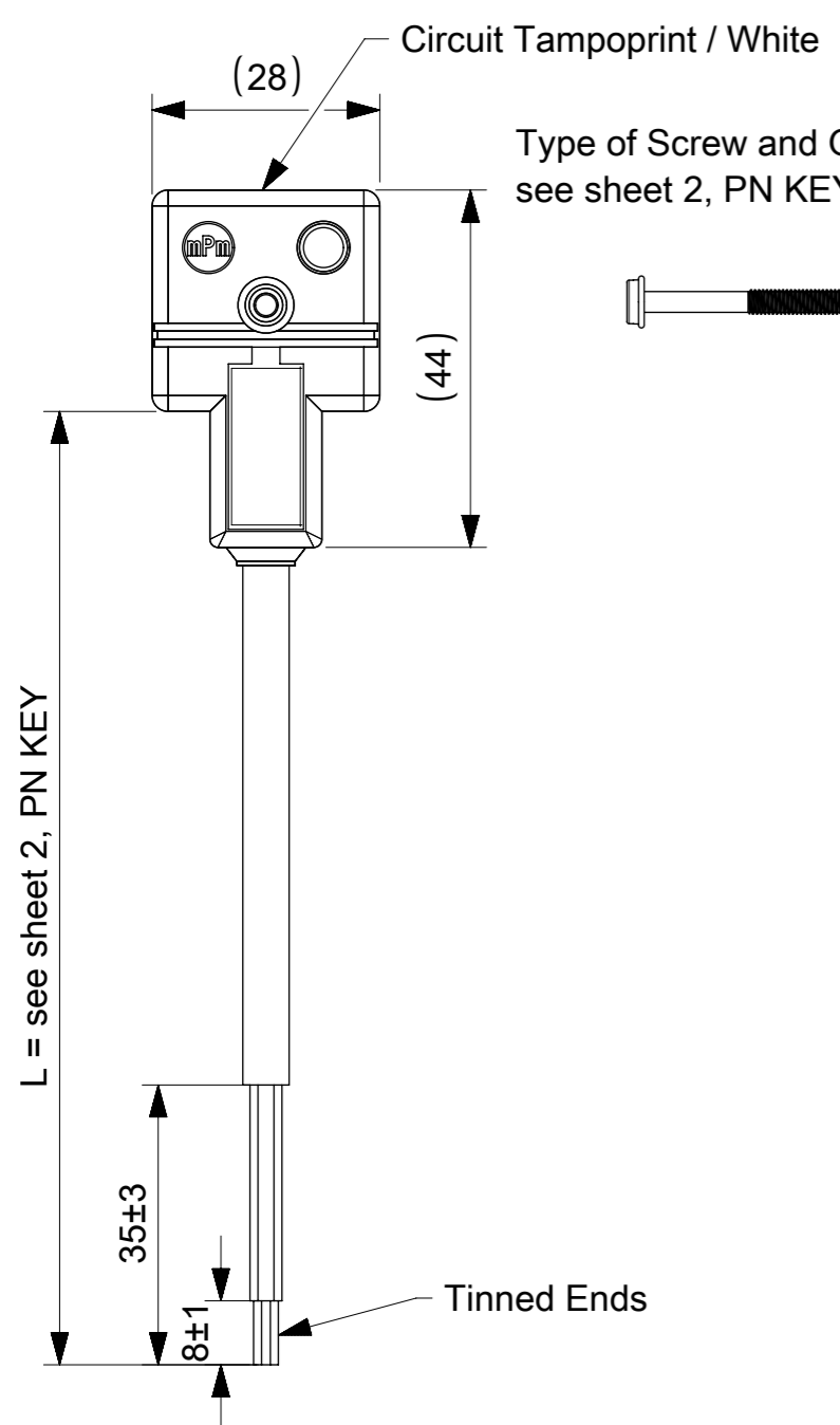
Type of Screws and Gaskets
