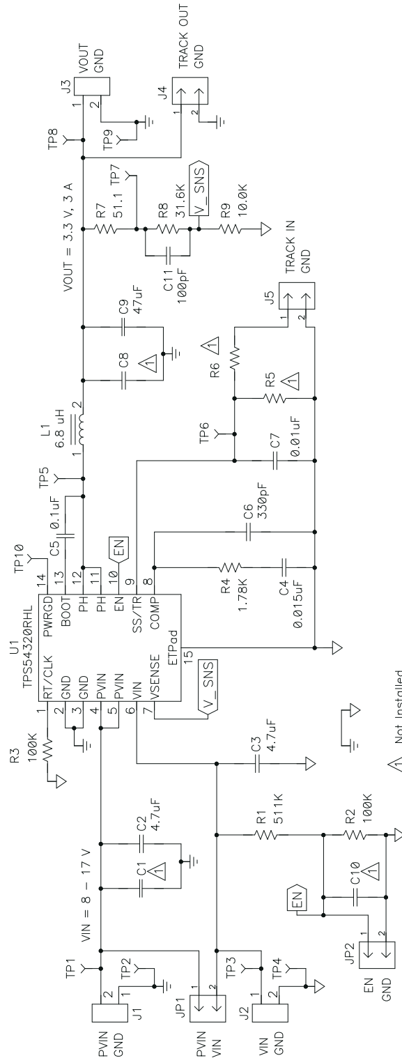
Figure 4-1. TPS54320EVm-513 Schematic
