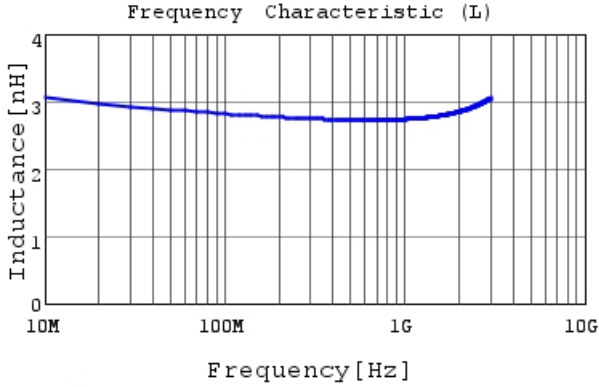
LQG15WH2N8B02 L
