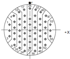
Contact Layout
