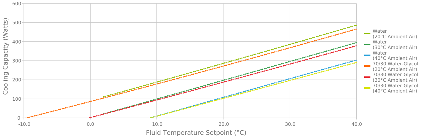
MRC300-DH2-HT-DV \Delta T (Inlet-Outlet) Fluid Temperature
