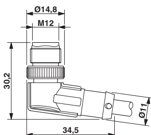
Plug M12 SPEEDCON, angled, shielded
