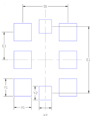
Figure 7.3. Si569 (2.5x3.2 mm) PCB Land Pattern
