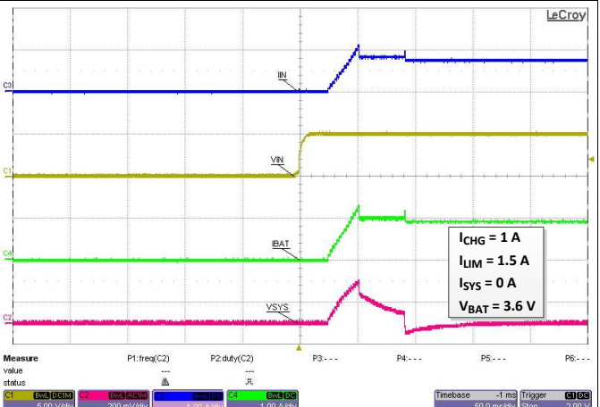
Figure 10. Startup
