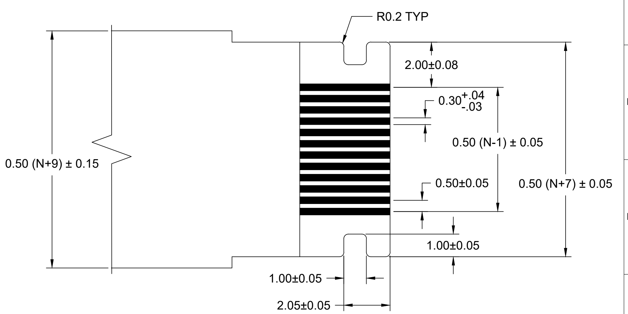
END-TAIL DIMENSIONS SCALE 10:1
