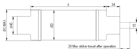
SJ Fuses
