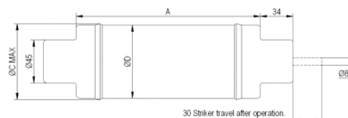
EJ Fuses
