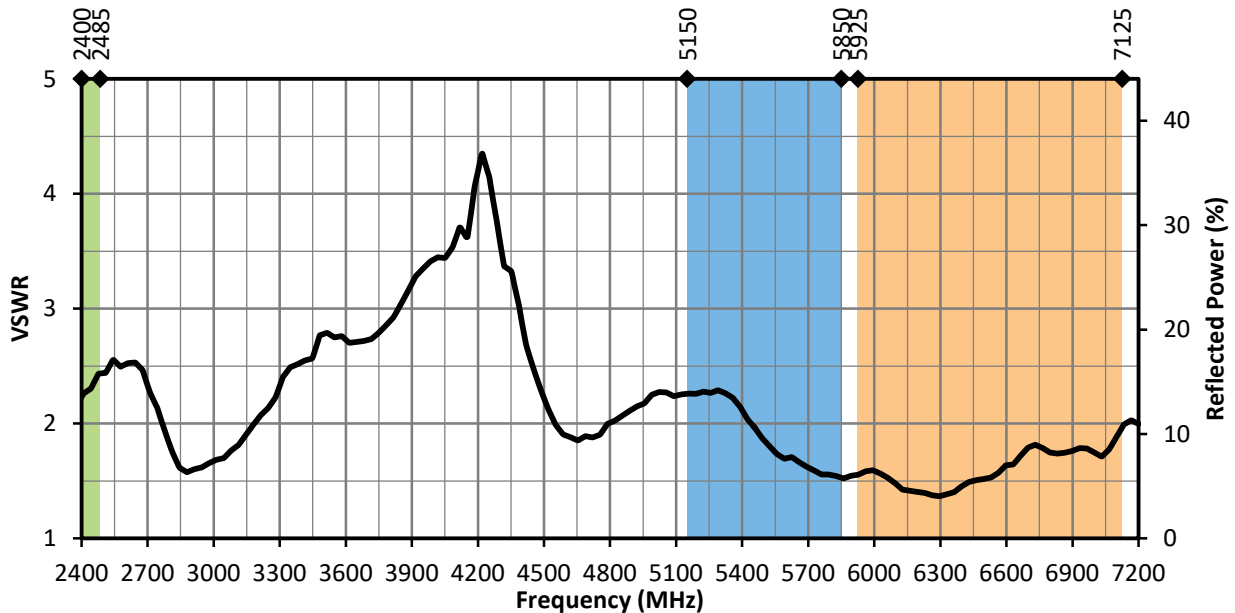
Figure 4. ANT-W63-MON VSWR, Edge-Bent
