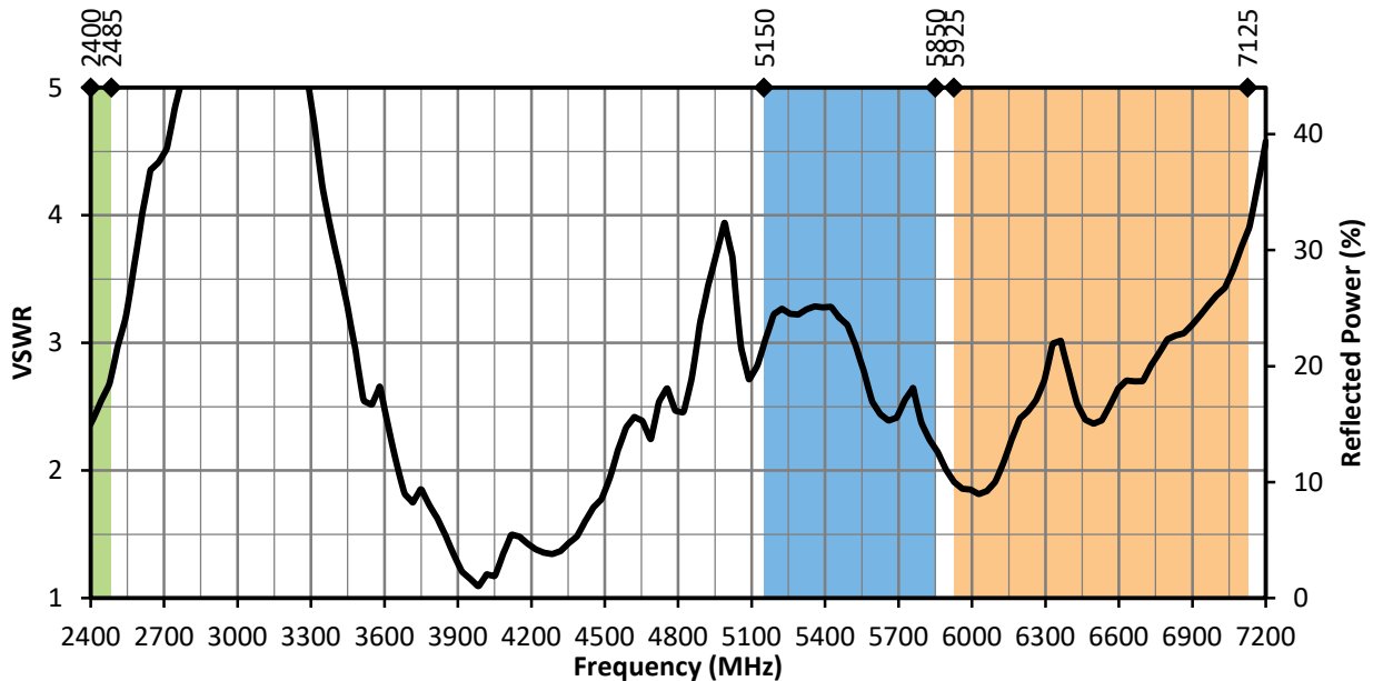
Figure 25. ANT-W63-MON VSWR, Straight
