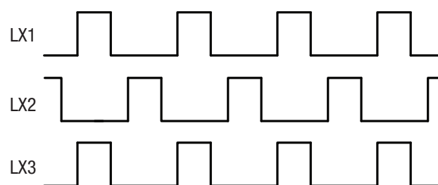
Figure 18. Out-of-Phase Operation
