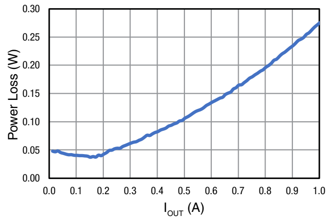
Figure 14. Channel 1 Power Loss at V_{IN} = 5\text{V} , No Airflow
