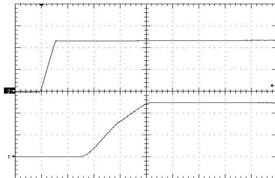
Figure 10. Startup Waveform via Input Voltage, time scale 4mS/div. Vin=Vin_nom, Iout=full load Cout=1000uF, Ch1=Vout (2V/div), Ch2=Vin (10V/div)
