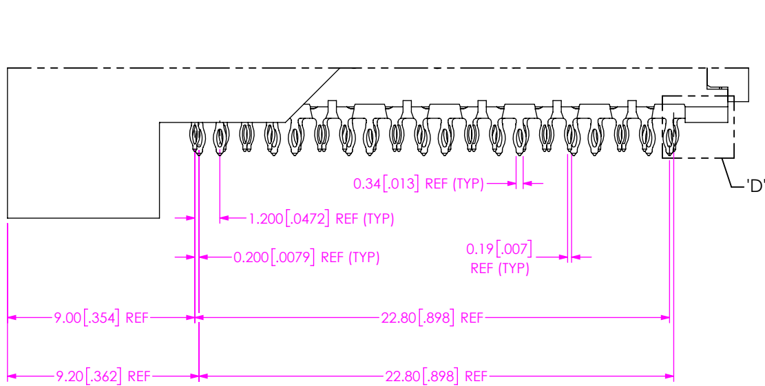
DETAIL 'C' SCALE 4 : 1
