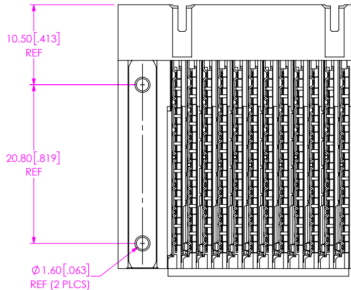
FIG 6 LEFT GUIDANCE EBTF-6-12-2.0-X-RA-X-L-A SHOWN (DIFFERENT AS SHOWN, OTHERWISE SAME AS FIG 5) (NOT RELEASED)
