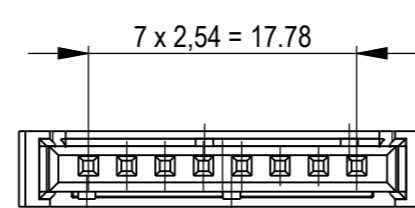
8-polige Variante/ 8-pole version Fabe: schwarz/ colour black
