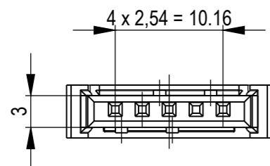
5-polige Variante/ 5-pole version Fabe: schwarz/ colour black
