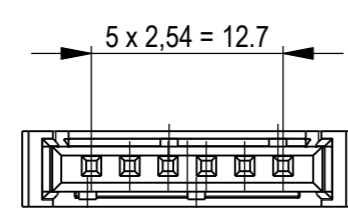
6-polige Variante/ 6-pole version Fabe: schwarz/ colour black
