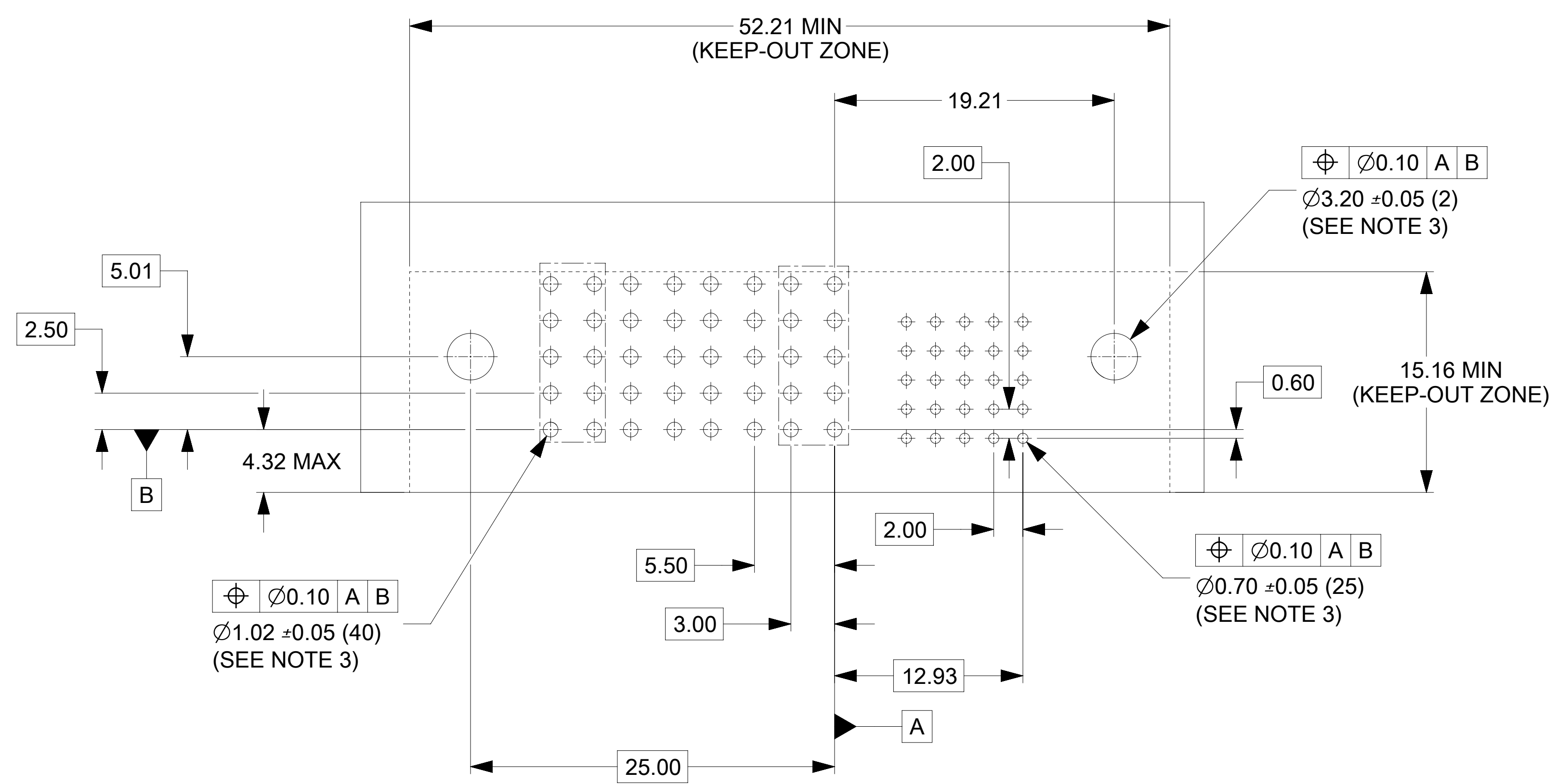
RECOMMENDED PCB LAYOUT AND KEEP-OUT ZONE
