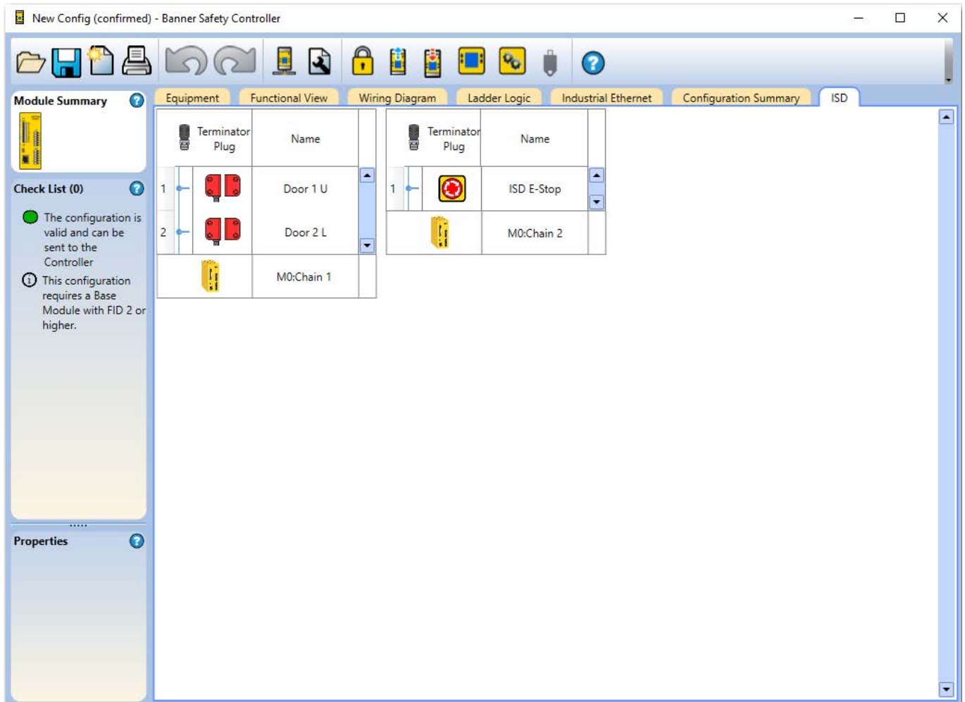
Figure 80. ISD Tab
