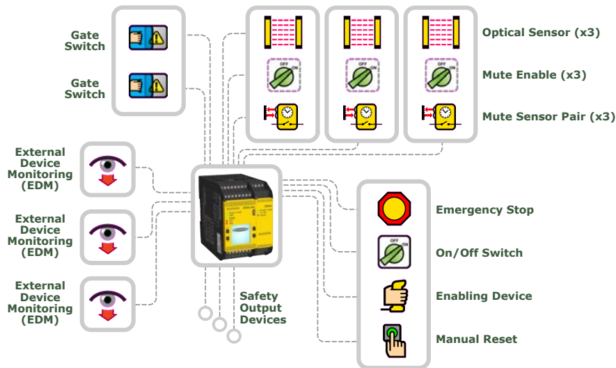
Figure 58. Sample Configuration Schematic
