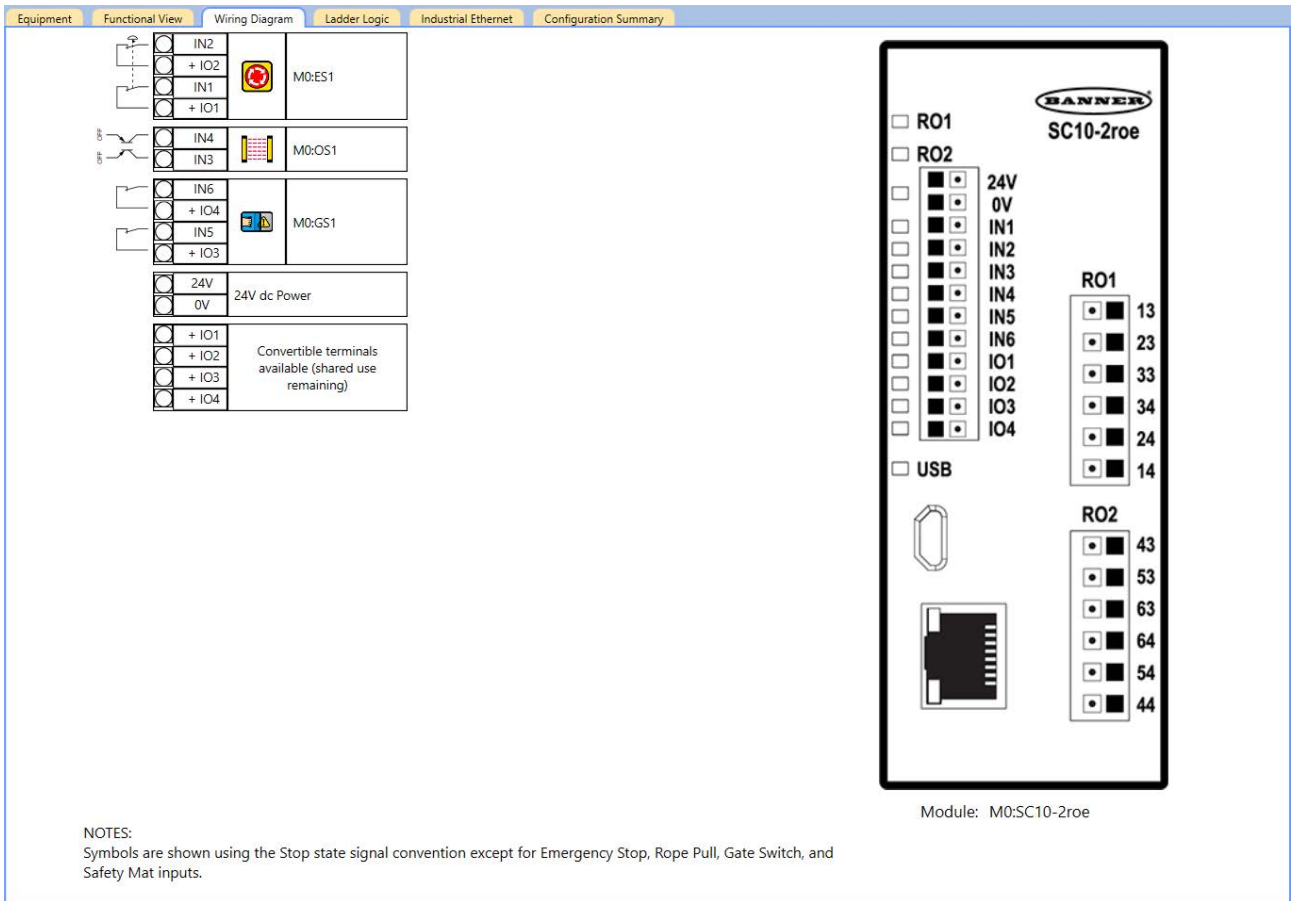
Figure 250. Wiring Diagram tab with an E-stop button, optical sensor, and gate switch
