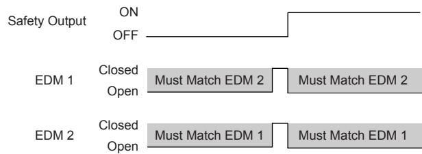
Figure 42. Timing logic: Two-channel EDM status, with respect to Safety Output
