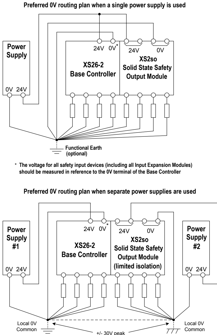
Figure 37. Wiring Diagram—Recommended Grounding
