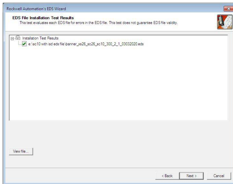
Figure 155. Register the Tested File
