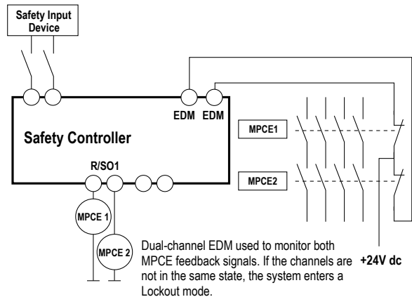
Figure 39. Two-channel EDM hookup
