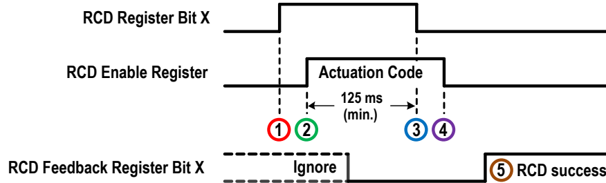
Figure 27. Virtual Reset or Cancel Delay (RCD) Sequence—Timed Method
