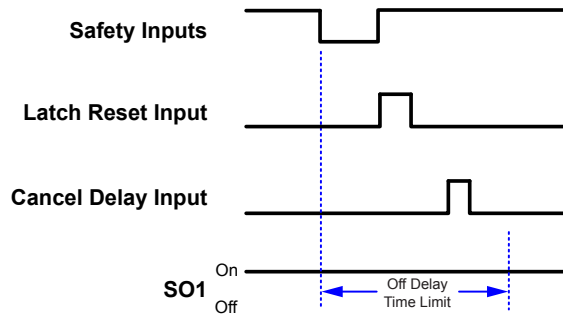
Figure 30. Keep Output On function for Safety Inputs with the Latch Reset
