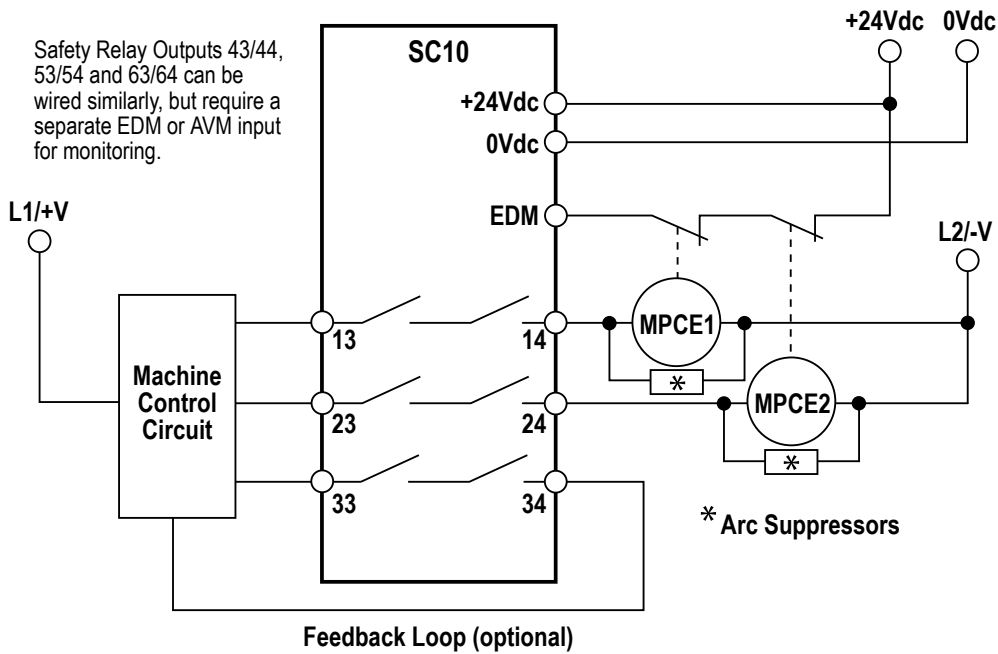
Figure 46. Generic SC10-2 Hookup: Safety Relay Output (Dual-Channel) with EDM
