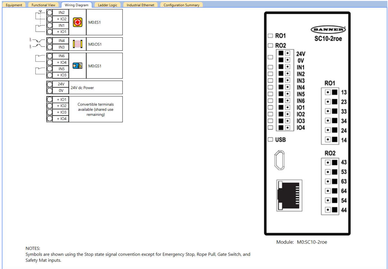
Figure 247. Wiring Diagram tab with an E-stop button, optical sensor, and gate switch
