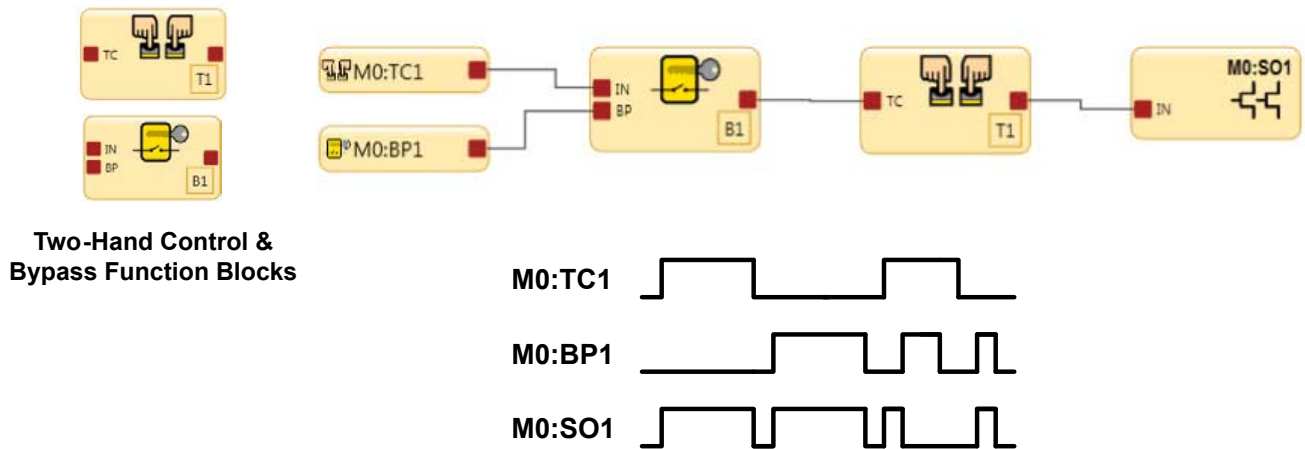
Figure 144. Timing Diagram—Two-Hand Control Block and Bypass Blocks with 1 Two-Hand Control Input
