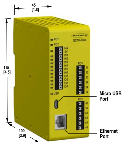
Figure 13. SC10-2 Dimensions
