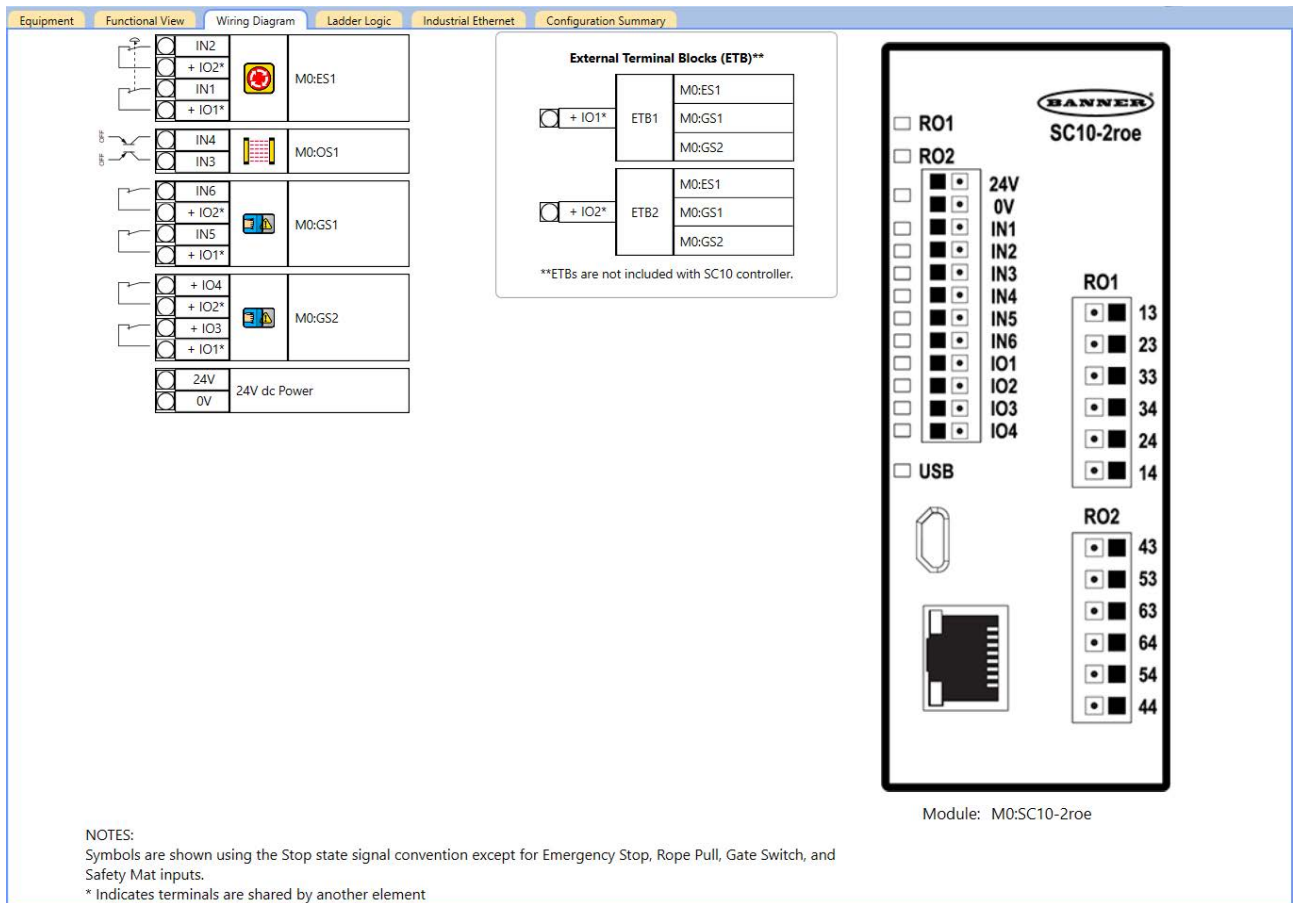
Figure 253. Wiring Diagram tab with an E-stop button, optical sensor, gate switches, and ETBs
