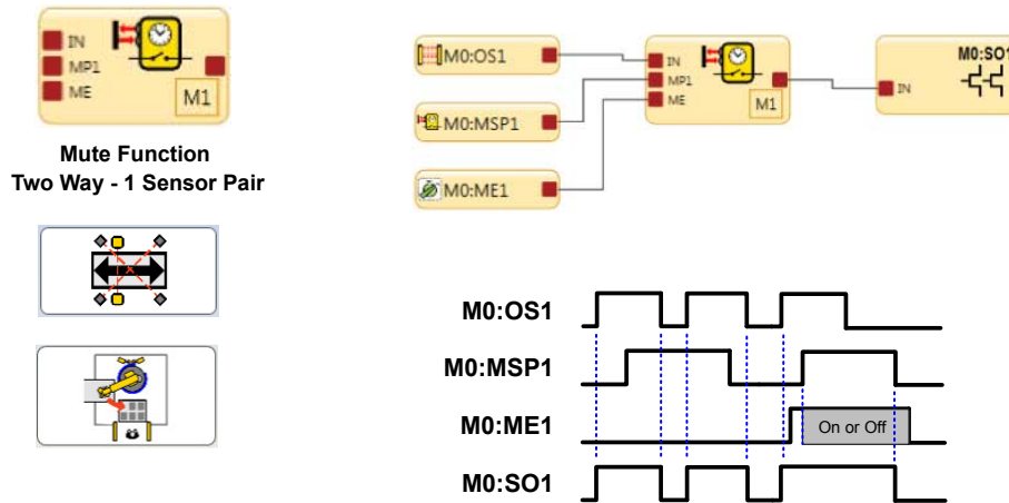
Figure 125. Timing Diagram—Two-Way Muting Block, One Muting Sensor Pair
