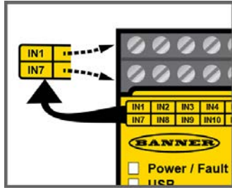
Figure 16. XS/SC26-2 Input and output terminal locations
