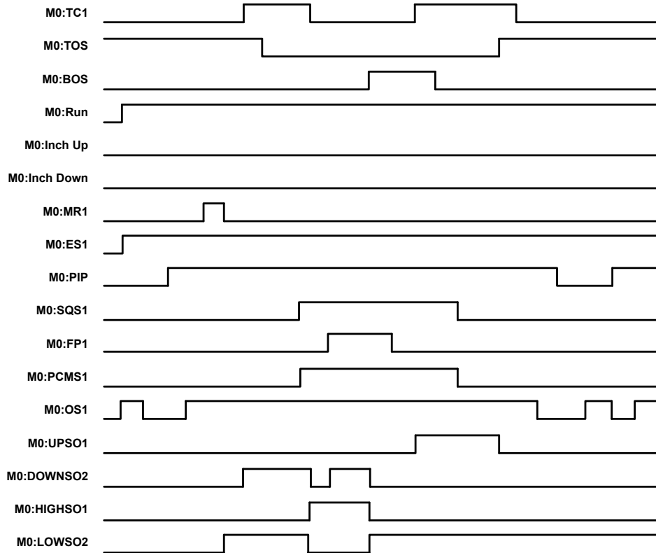
Figure 140. Press Control—Timing Diagram with Manual Upstroke Setting
