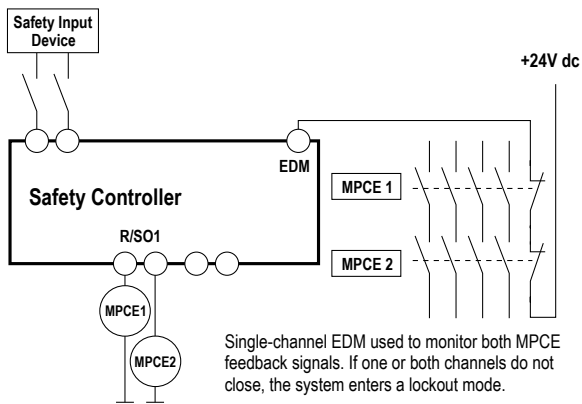
Figure 38. One-channel EDM hookup
