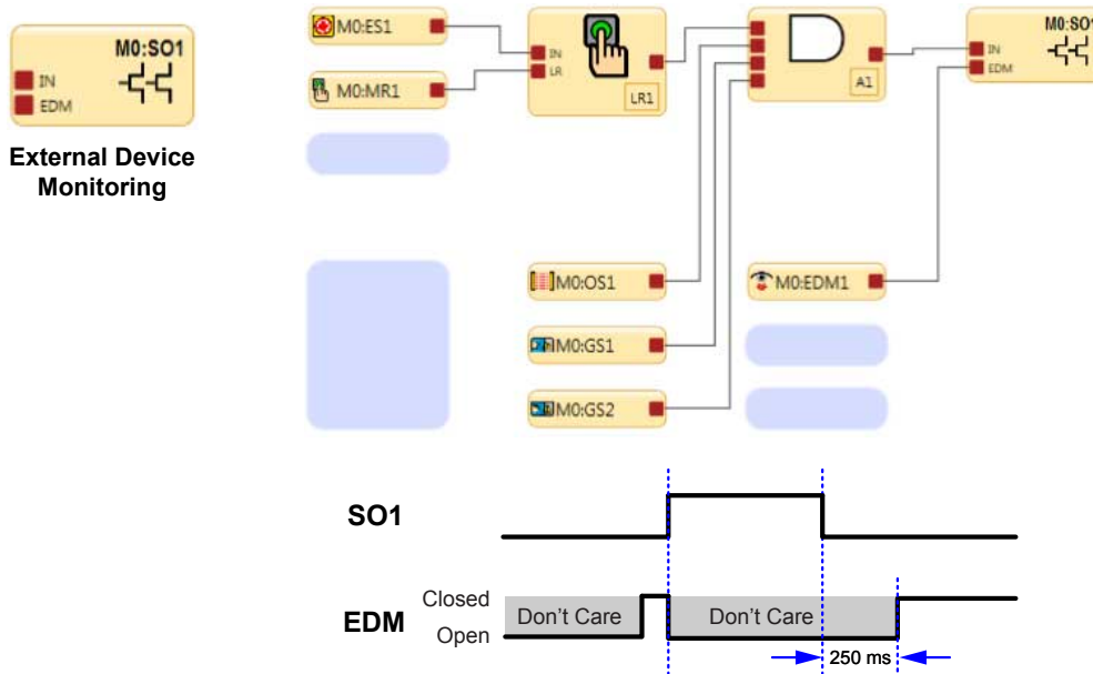
Figure 40. Timing logic: One-channel EDM status, with respect to Safety Output
