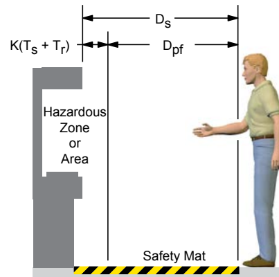
Figure 19. Determining safety distance for the safety mat
