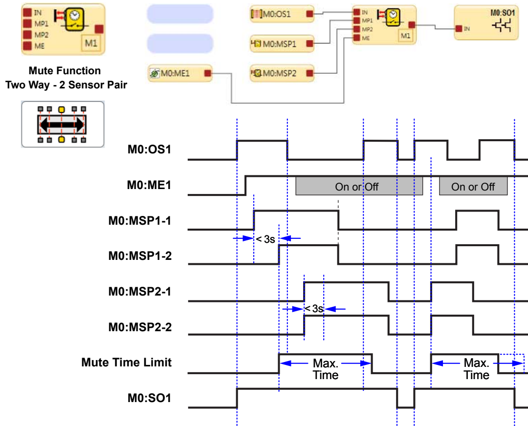
Figure 126. Timing Diagram—Two-Way Muting Block, Two Muting Sensor Pairs
