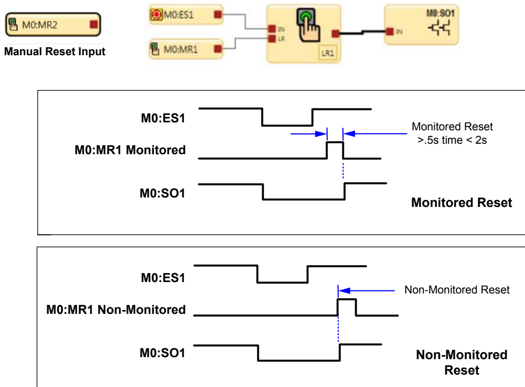
Figure 115. Timing Diagram—Latch Reset Block, Monitored/Non-Monitored Reset
