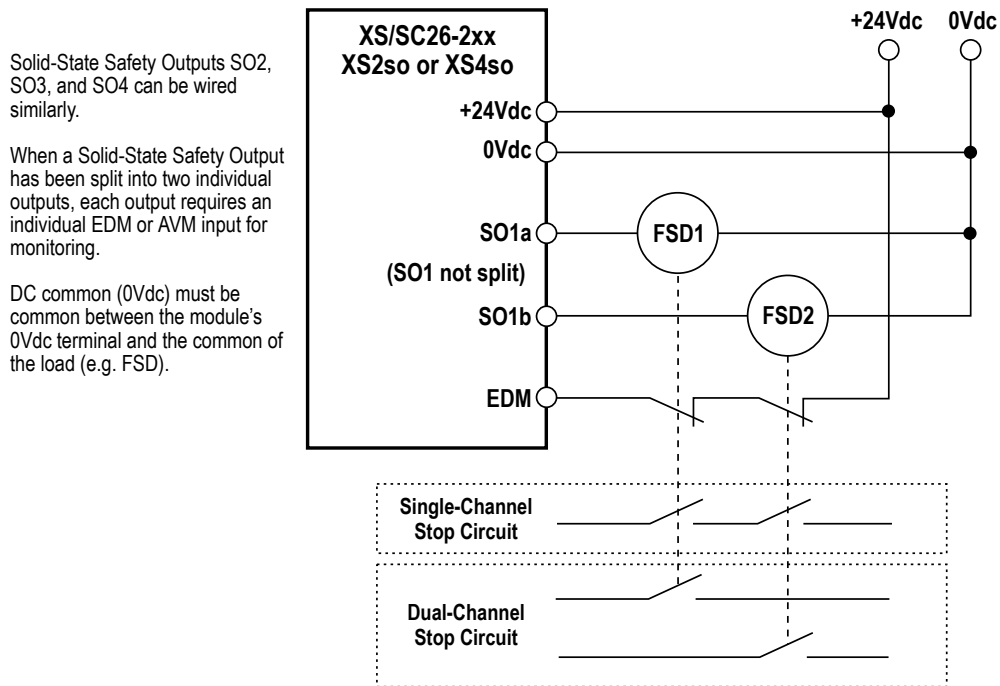
Figure 43. Generic XS/SC26-2 Hookup: Solid-State Safety Output with EDM
