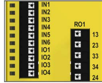
Figure 17. SC10-2 Input and output terminal locations
