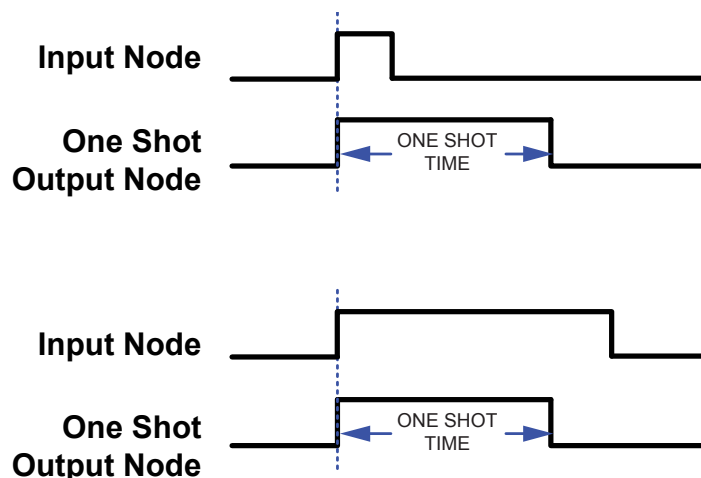
Figure 130. Typical Normal One Shot Timing Diagrams
