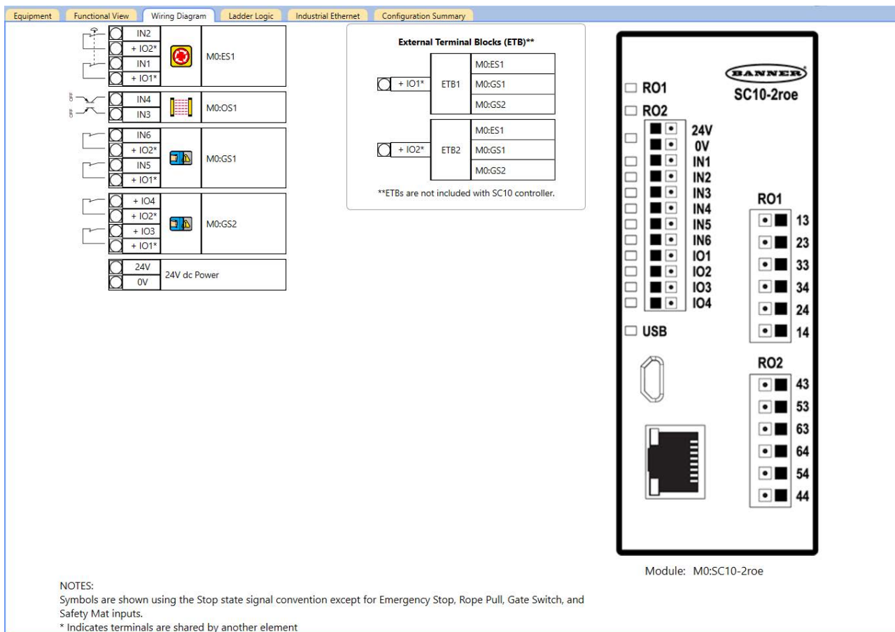
Figure 248. Wiring Diagram Tab with Three E-stop Buttons and ETBs
