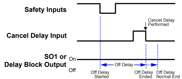
Figure 31. Keep Output On function for Safety Inputs without the Latch Reset
