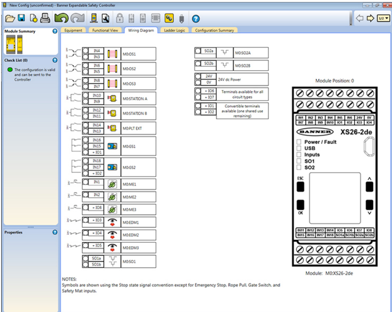
Figure 77. Wiring Diagram Tab—XS26-2
