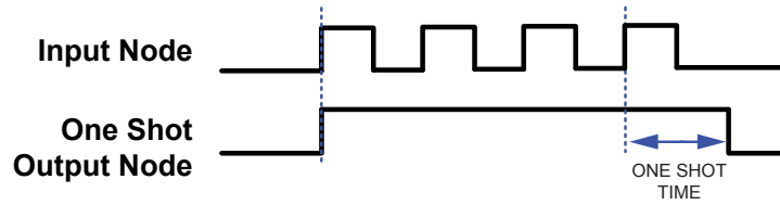
Figure 131. Heartbeat One Shot Timing Diagram
