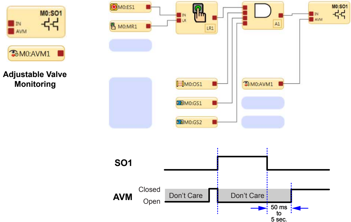
Figure 20. Timing logic—AVM Function
