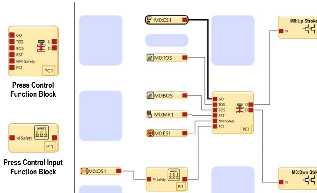
Figure 137. Sample Configuration for a Small Press
