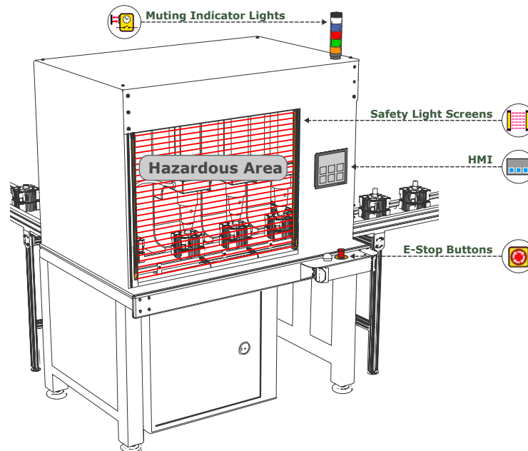
Figure 15. SC10-2 Sample Application
