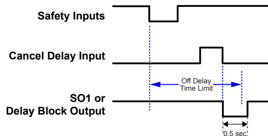
Figure 29. Turn Output Off function
