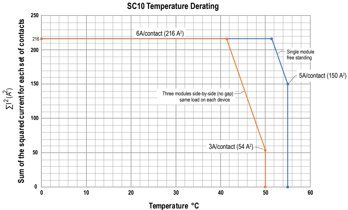
Figure 10. SC10-2 Temperature Derating
