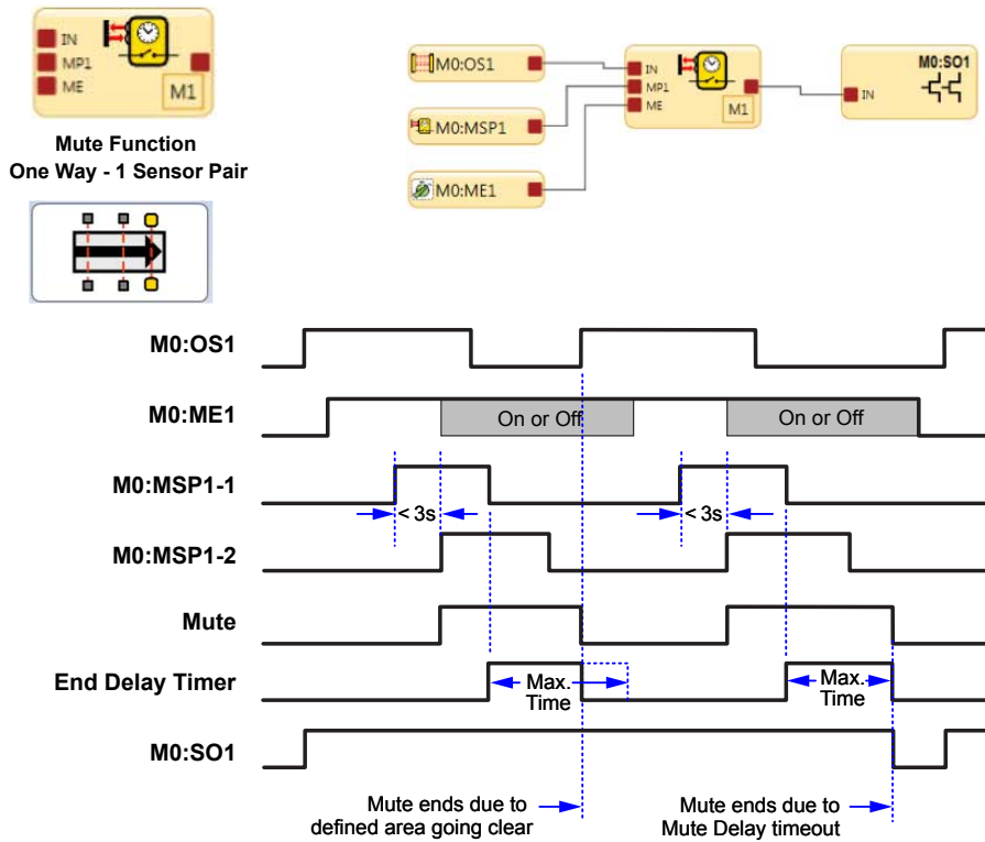
Figure 123. Timing Diagram—One-Way Muting Block, One Muting Sensor Pair
