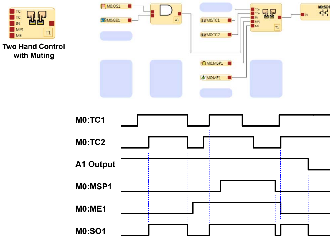
Figure 147. Timing Diagram—Two-Hand Control Block with Muting
