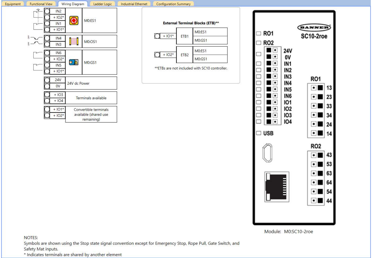
Figure 252. Wiring Diagram tab with an E-stop button, optical sensor, gate switch, and ETBs
