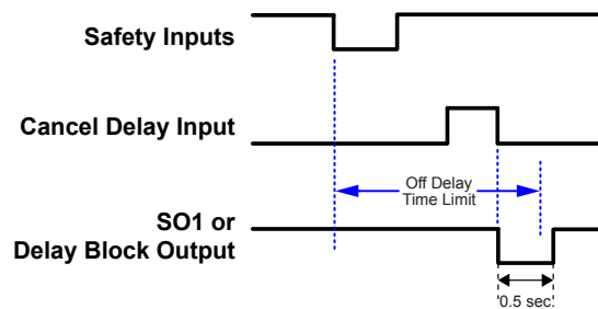
Figure 22. Turn Output Off function
