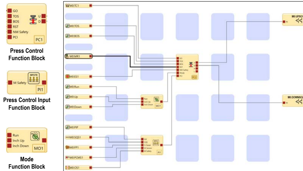
Figure 139. Press Control—Sample Configuration
