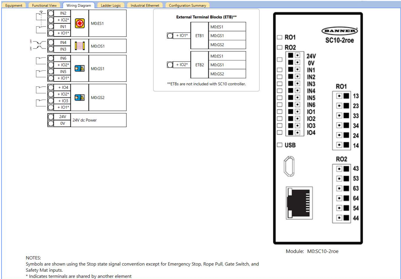
Figure 78. Wiring Diagram Tab—SC10-2 with External Terminal Blocks
