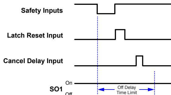
Figure 23. Keep Output On function for Safety Inputs with the Latch Reset
