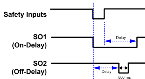
Figure 32. Timing Diagram—General Safety Output On-Delay and Off-Delay
