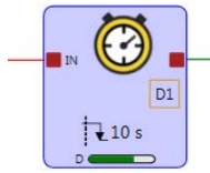
Figure 106. Delay Block—XS/SC26-2 FID 2 or later Base Controllers only and SC10-2
