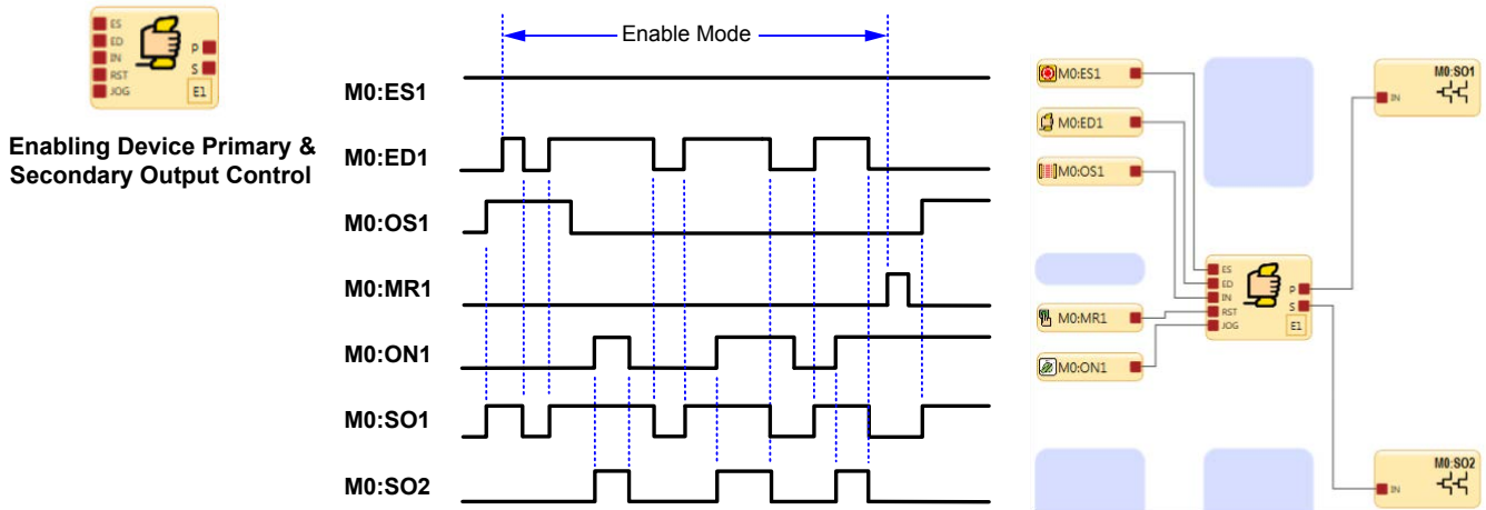
Figure 113. Timing Diagram—Enabling Device
