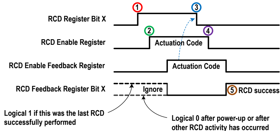
Figure 26. Virtual Reset or Cancel Delay (RCD) Sequence—Feedback Method
