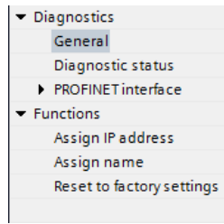
Figure 239. Online & Diagnostics
