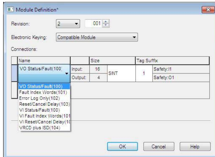
Figure 161. Module Definition
