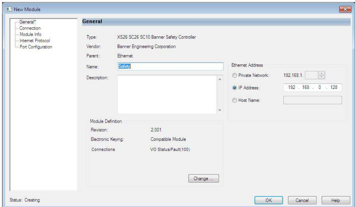
Figure 160. New Module
