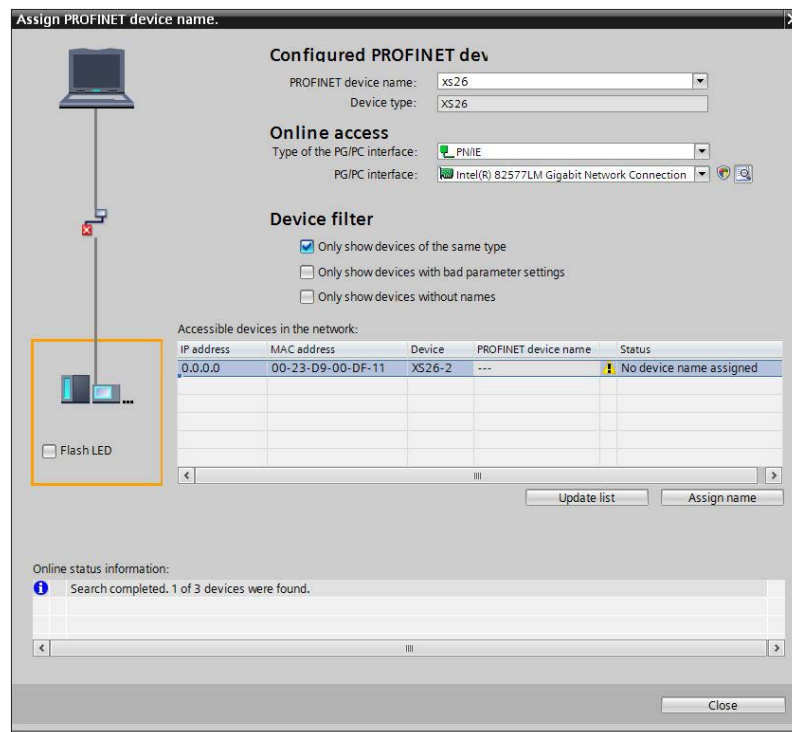
Figure 245. Ethernet Addresses
