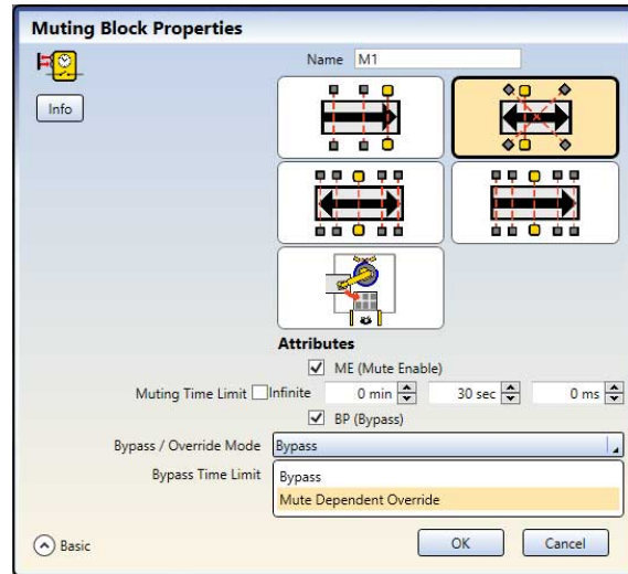
Figure 121. Mute-Dependent Override
