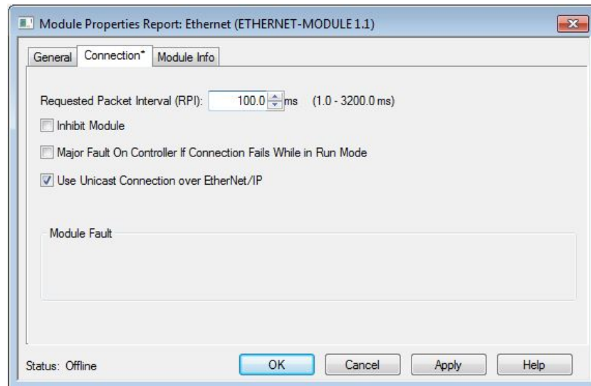
Figure 179. Connection Parameters
