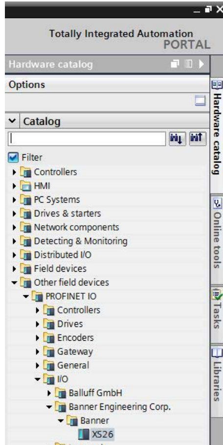
Figure 234. Hardware Catalog
