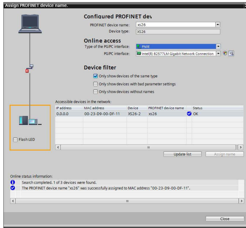
Figure 246. Ethernet Addresses
