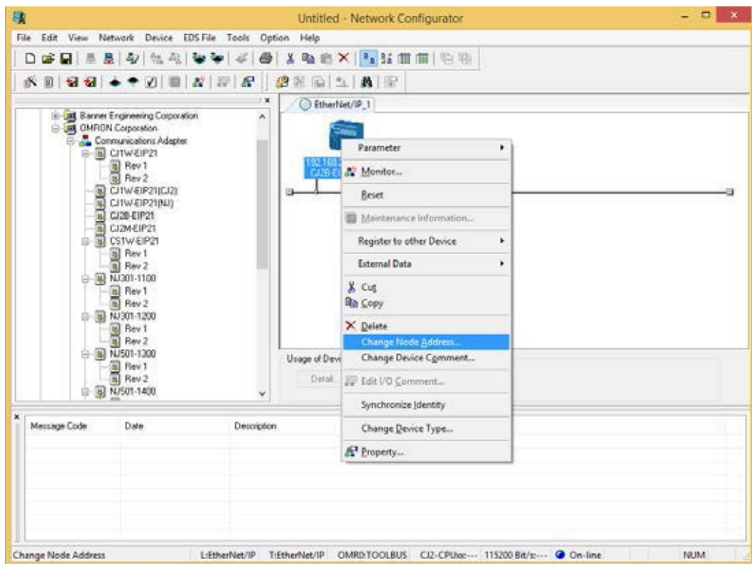
Figure 199. Right-Click Menu
