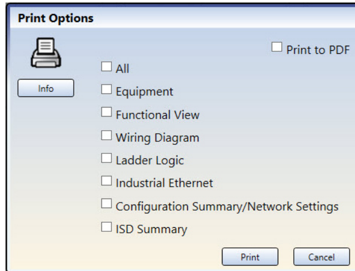
Figure 90. Print Options
