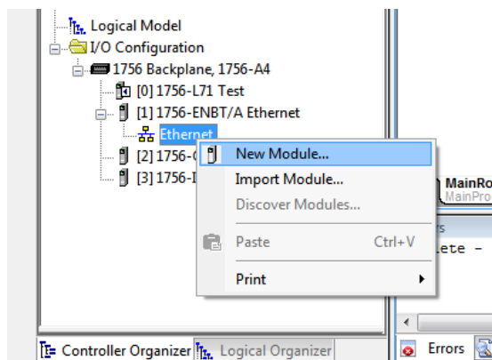
Figure 158. New Module
