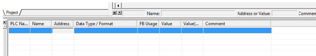
Figure 223. Watch Window
