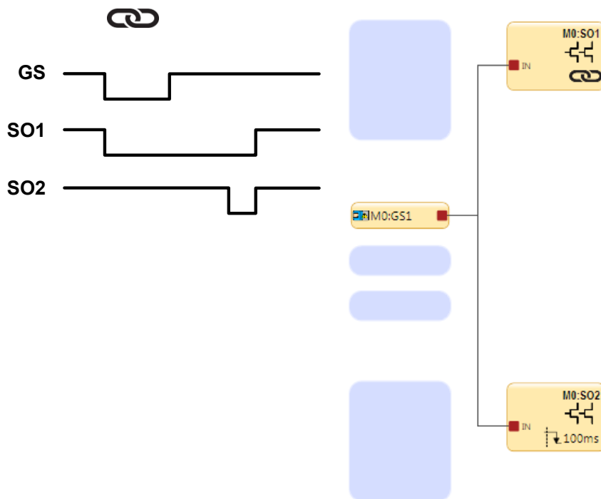
Figure 35. Timing Diagram—Linked Safety Outputs
