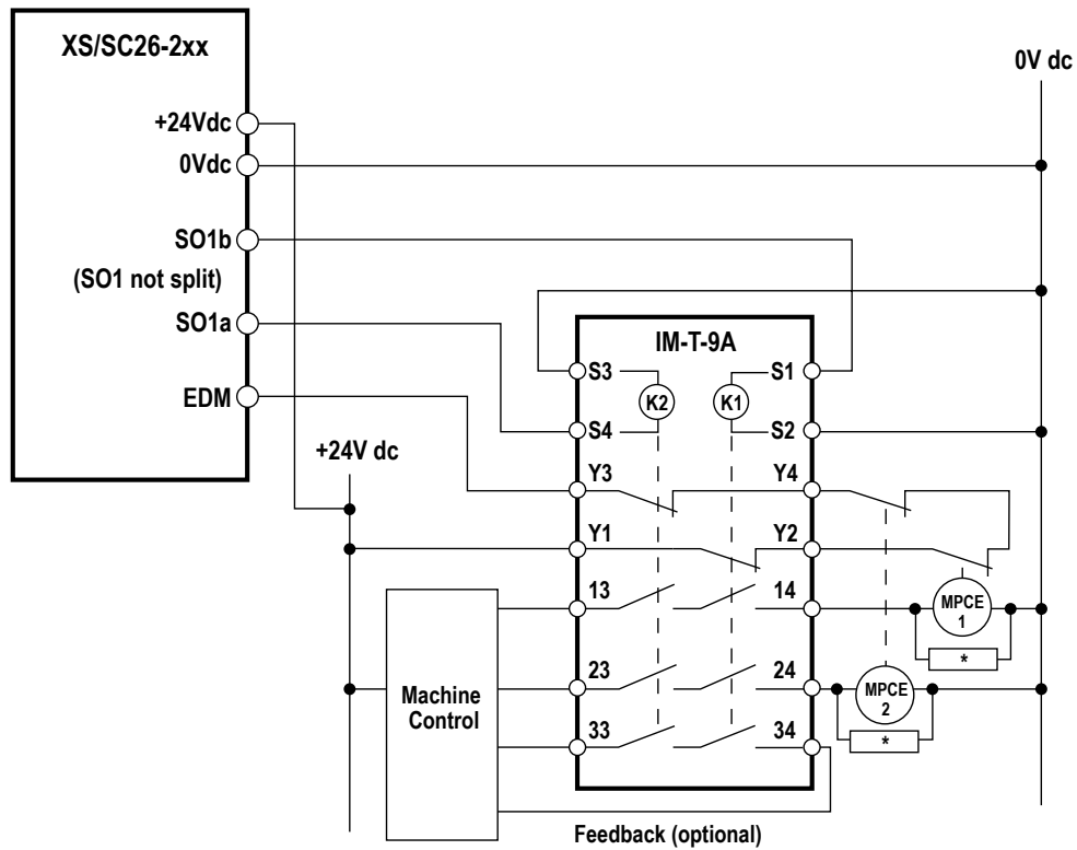
Figure 45. Generic XS/SC26-2 Hookup: Solid-State Safety Output to IM-T-9A
