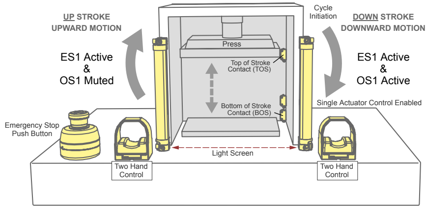
Figure 60. Simple Sample Press Control Configuration
