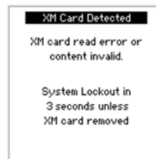
Figure 272. SC-XM2/3 Error
