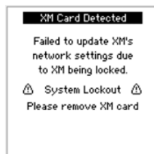
Figure 267. System Lockout
