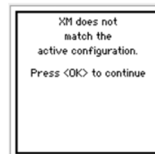
Figure 262. Mismatch
