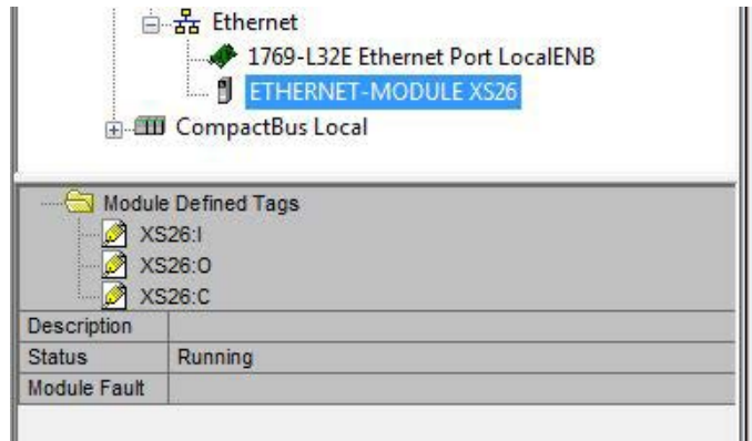
Figure 180. Successful Configuration
