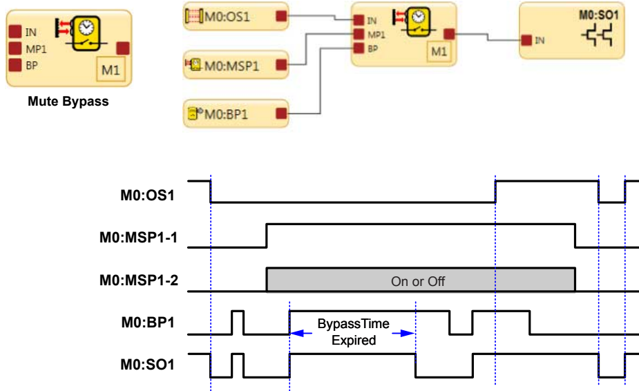
Figure 122. Mute Bypass
