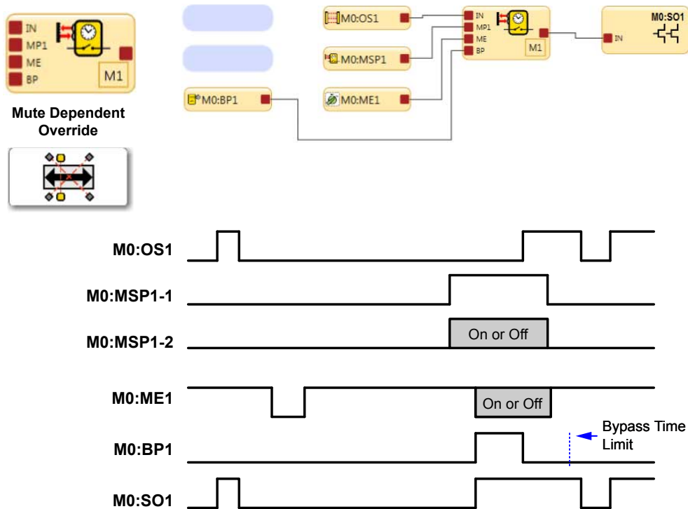
Figure 121. Mute-Dependent Override
