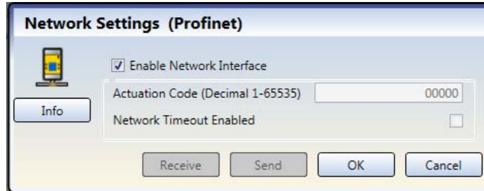
Figure 86. Network Settings—PROFINET
