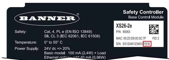
Figure 151. Serial Number
