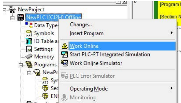
Figure 222. Work Online
