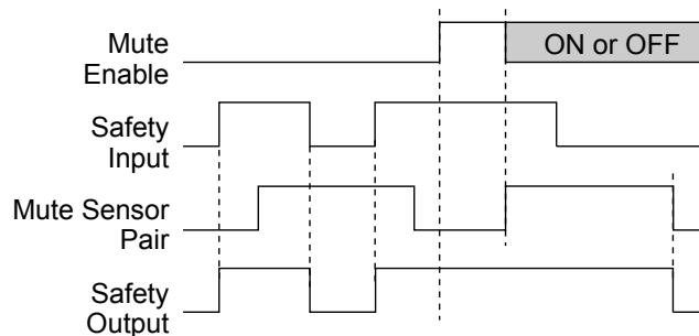
Figure 128. Timing logic—One mute sensor pair with mute enable
