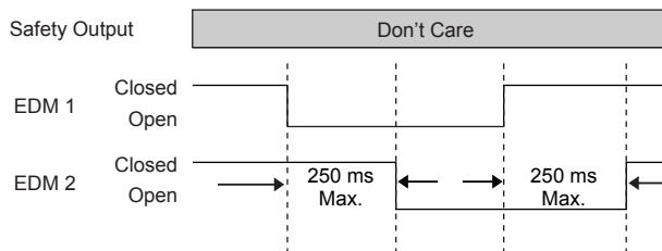
Figure 41. Timing logic: Two-channel EDM, timing between channels
