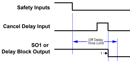
Figure 21. Safety Input remains in Stop mode
