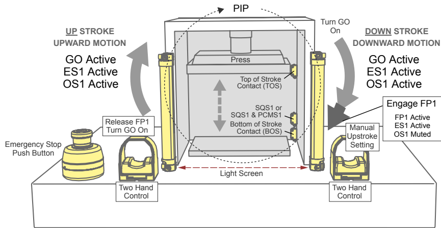
Figure 64. Full Feature Sample Press Control Configuration
