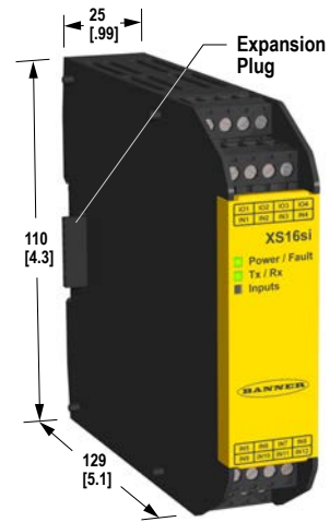
Figure 12. Expansion Module Dimensions
