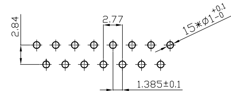
15 Pin Female Connector PCB Pin Layout Scale 2:1
