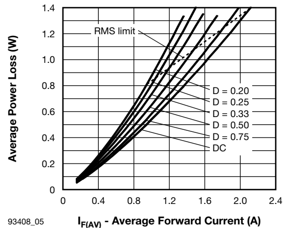
93408_05 I F(AV) - Average Forward Current (A) Fig. 5 - Maximum Average Forward Dissipation vs. Average Forward Current
