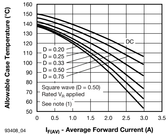
93408_04 I F(AV) - Average Forward Current (A) Fig. 4 - Maximum Average Forward Current vs. Allowable Lead Temperature
