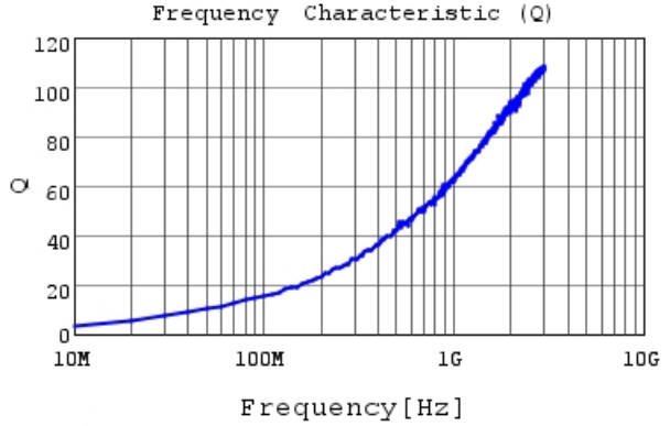
LQG15WZ1N4B02 Q
