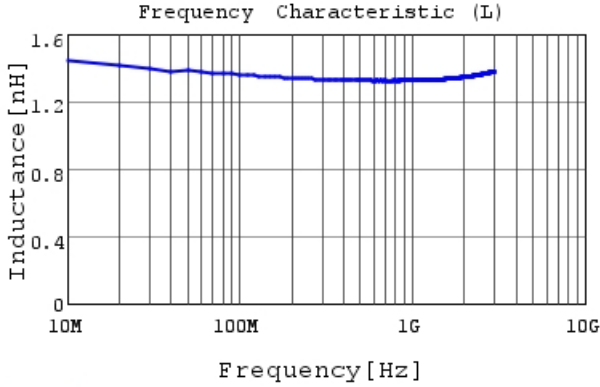
LQG15WZ1N4B02 L
