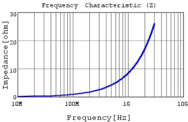
LQG15WZ1N4B02 |Z|
