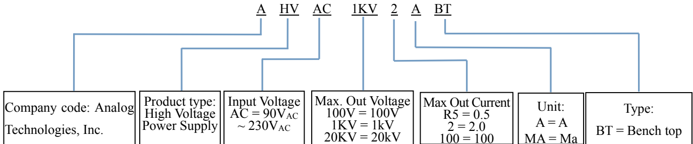
Figure 6. Naming Rules of AHVAC1KV2ABT
