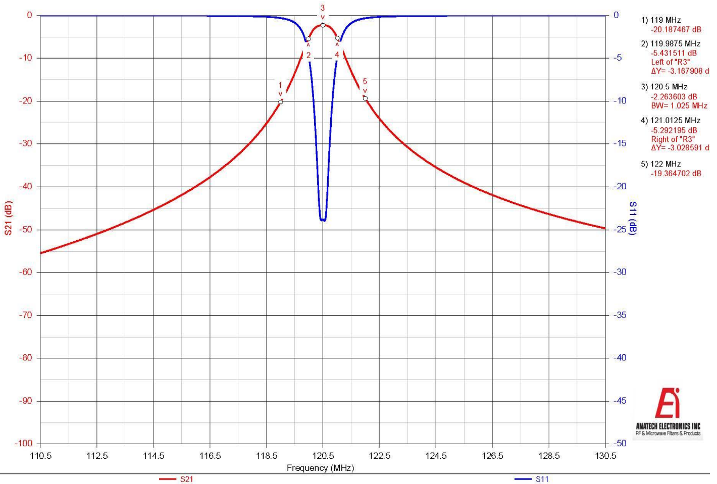
RFQ-20171110-BPF-120R5-1 MHz
