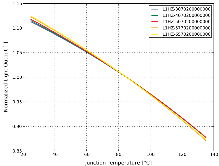
Figure 4. Typical normalized light output vs. junction temperature for LUXEON HL2Z 70 CRI at 700mA.
