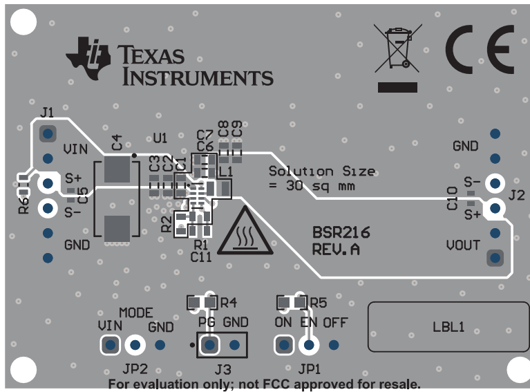
Figure 5-1. Top Assembly
