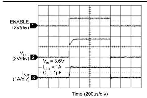
FIGURE 2-17: MIC94162/3 Start-Up ( I_{OUT} = 1A ).
