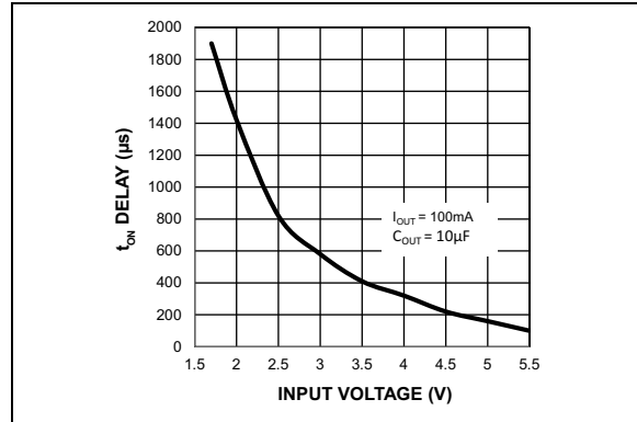
FIGURE 2-16: t_{ON} Delay vs. Input Voltage (MIC94161/4/5).
