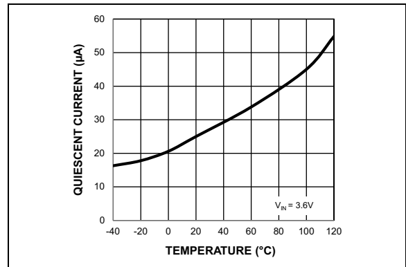
FIGURE 2-11: Quiescent Current vs. Temperature (MIC94162/3).
