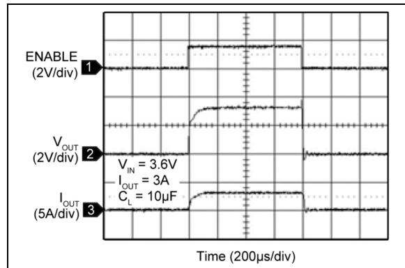
FIGURE 2-18: MIC94162/3 Start-Up ( I_{OUT} = 3A ).
