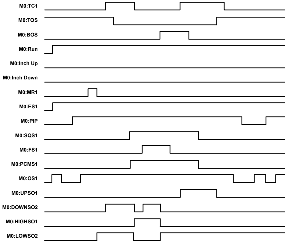
Figure 148. Press Control—Timing Diagram with Manual Upstroke Setting
