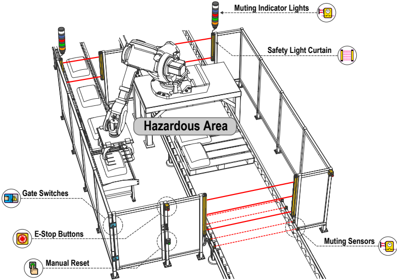
Figure 18. Sample Application - Robotic Cell
