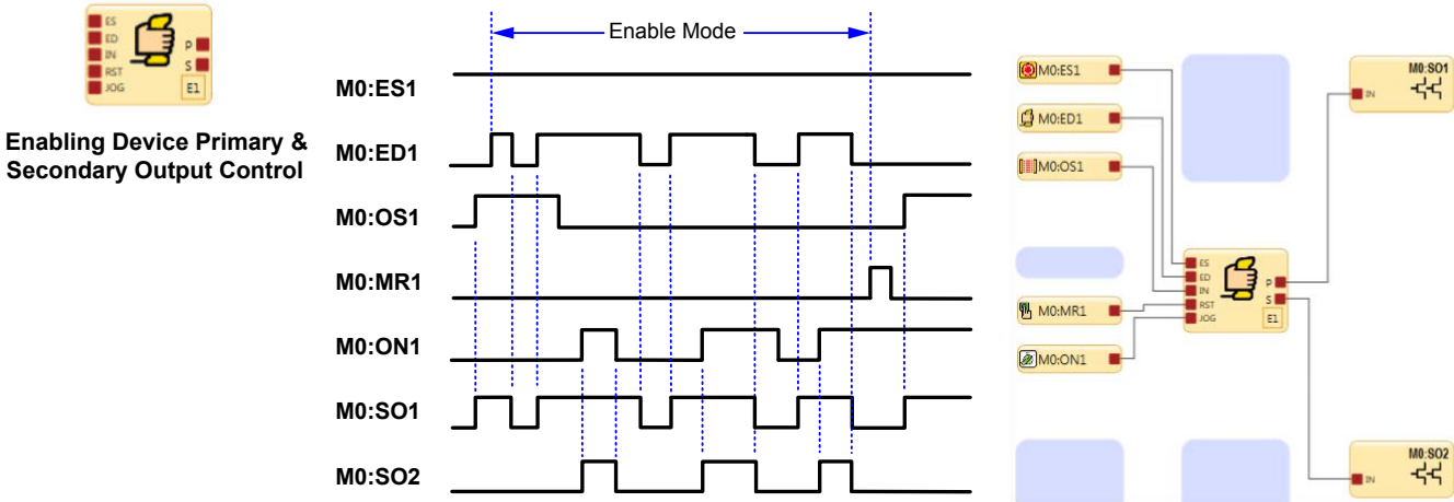
Figure 122. Timing Diagram—Enabling Device
