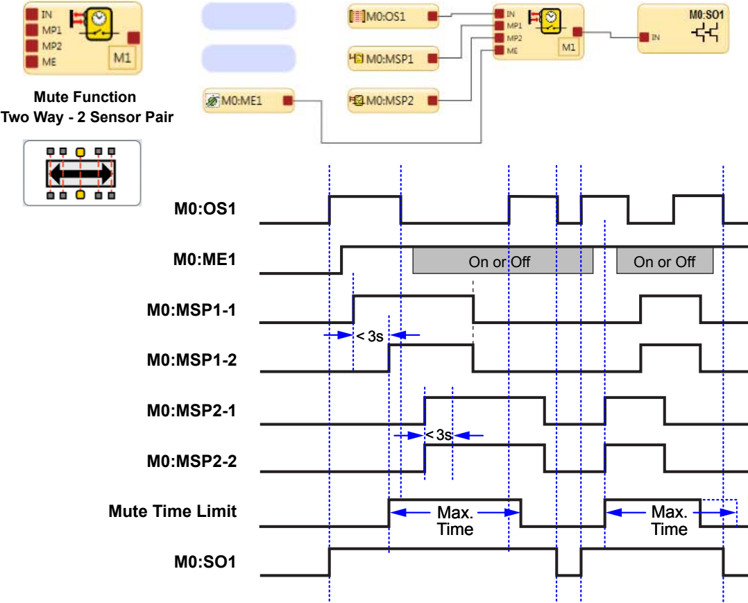
Figure 135. Timing Diagram—Two-Way Muting Block, Two Muting Sensor Pairs
