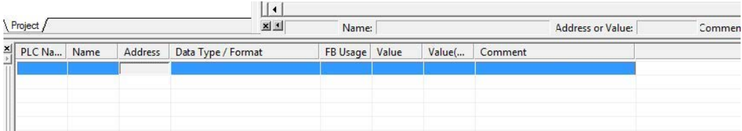
Figure 245. Watch Window
