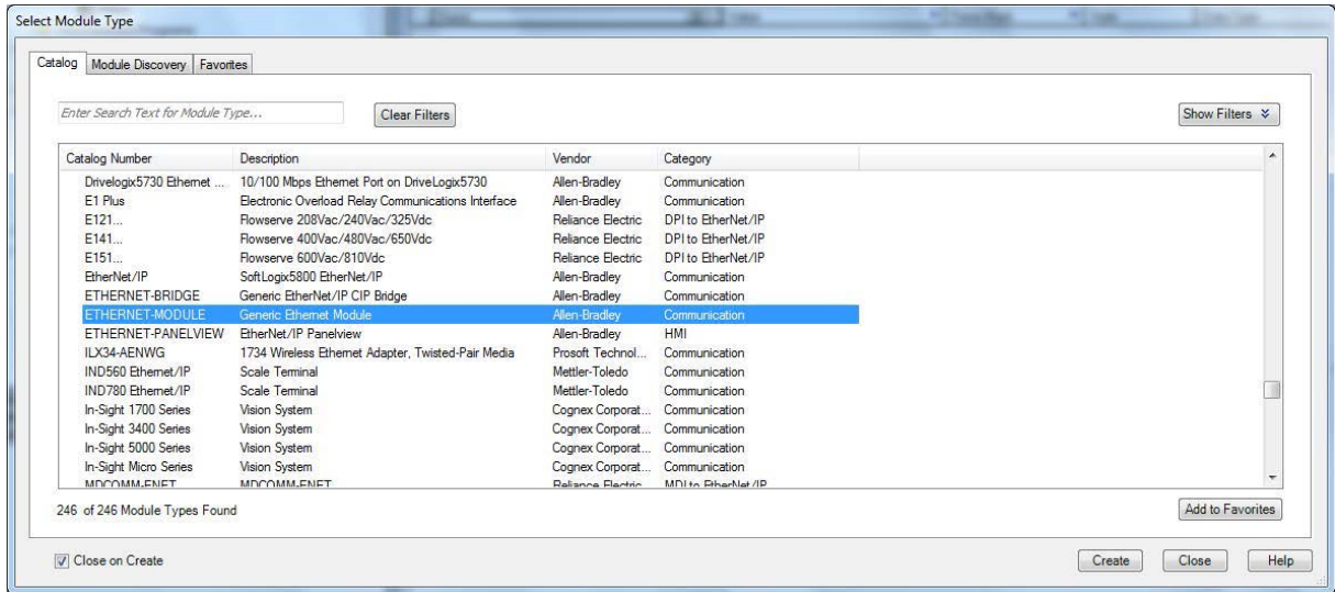
Figure 189. Select Module
