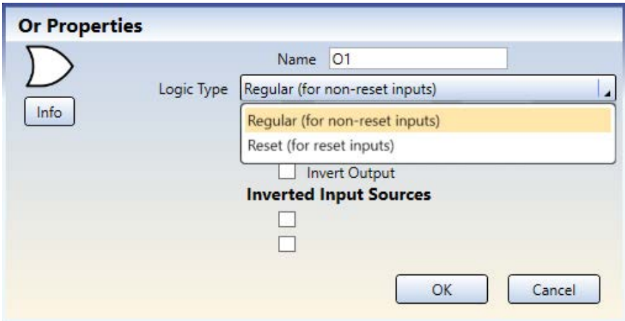
Figure 83. Or Properties
