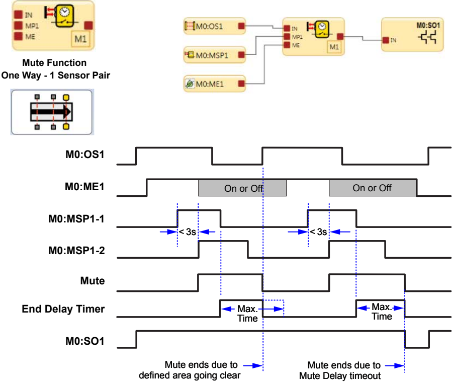
Figure 132. Timing Diagram—One-Way Muting Block, One Muting Sensor Pair
