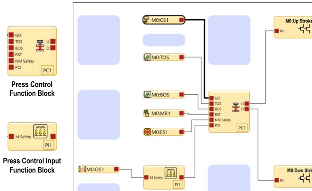
Figure 145. Sample Configuration for a Small Press
