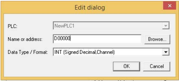
Figure 246. Edit Dialog
