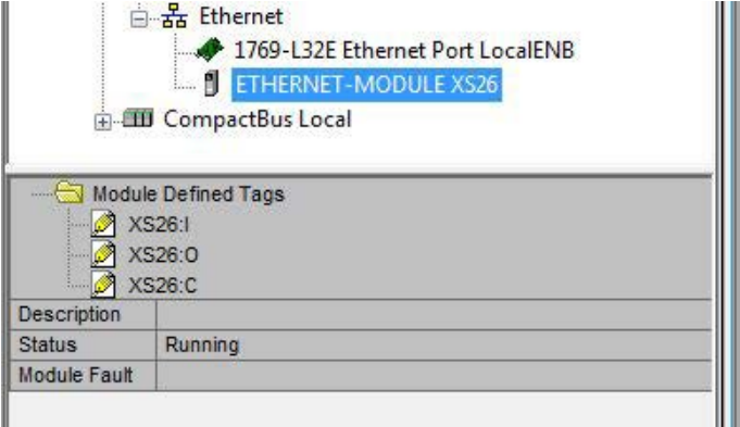
Figure 202. Successful Configuration
