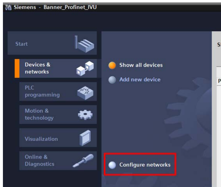
Figure 255. Configure Networks
