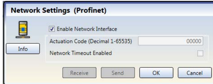
Figure 96. Network Settings—PROFINET
