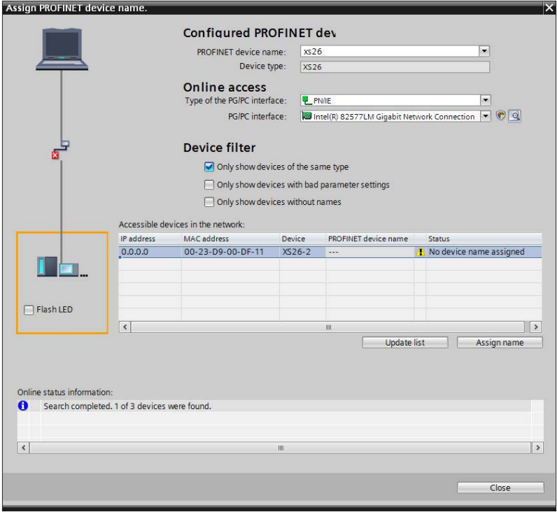
Figure 278. Ethernet Addresses
