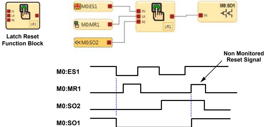
Figure 123. Timing Diagram—Latch Reset Block
