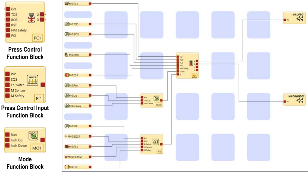
Figure 147. Press Control—Sample Configuration
