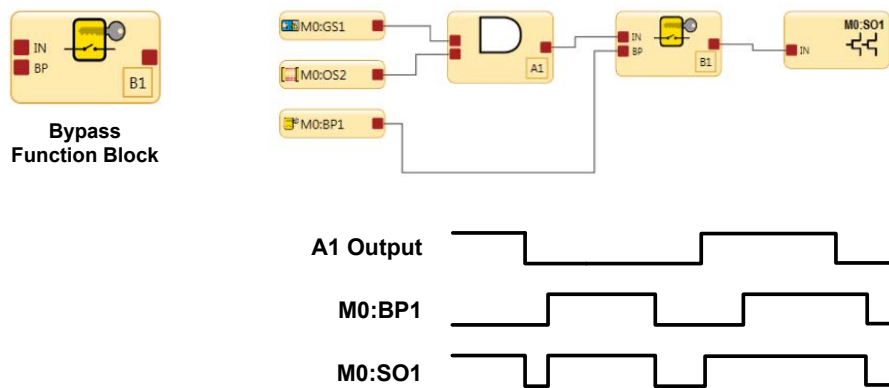
Figure 118. Timing Diagram—Bypass Block
