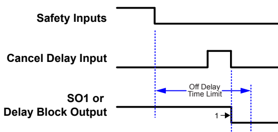
Figure 26. Safety Input remains in Stop mode
