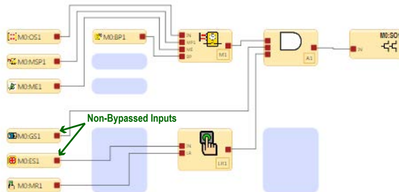
Figure 288. Mute Function with Bypass
