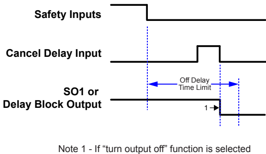
Figure 33. Safety Input remains in Stop mode
