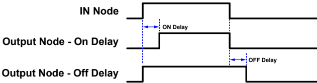
Figure 119. Delay Block Timing Diagram
