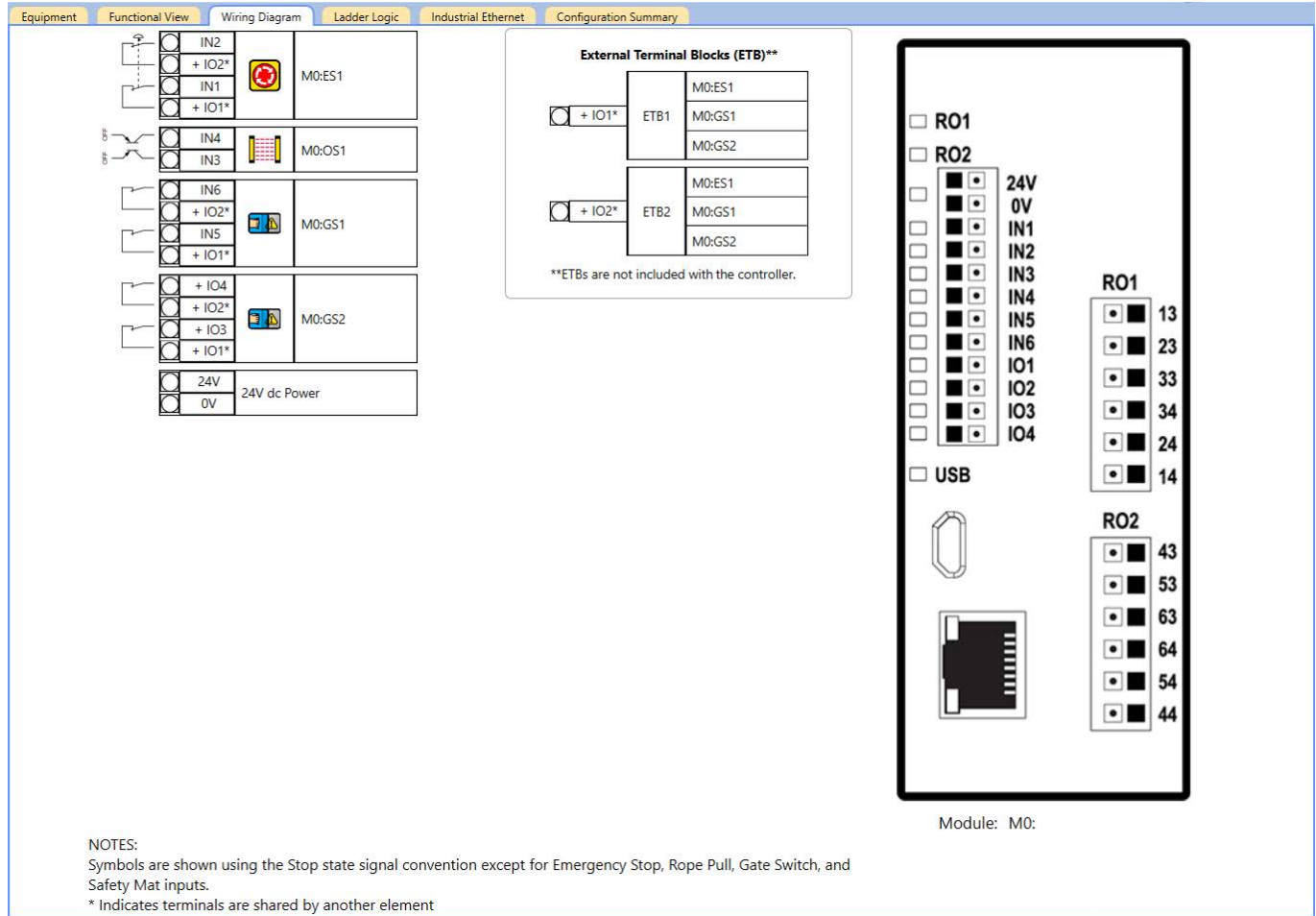
Figure 300. Wiring Diagram tab with an E-stop button, optical sensor, gate switches, and ETBs
