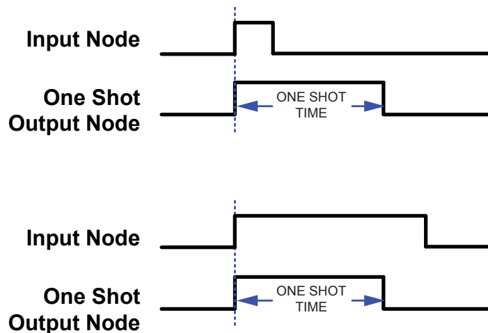
Figure 138. Typical Normal One Shot Timing Diagrams
