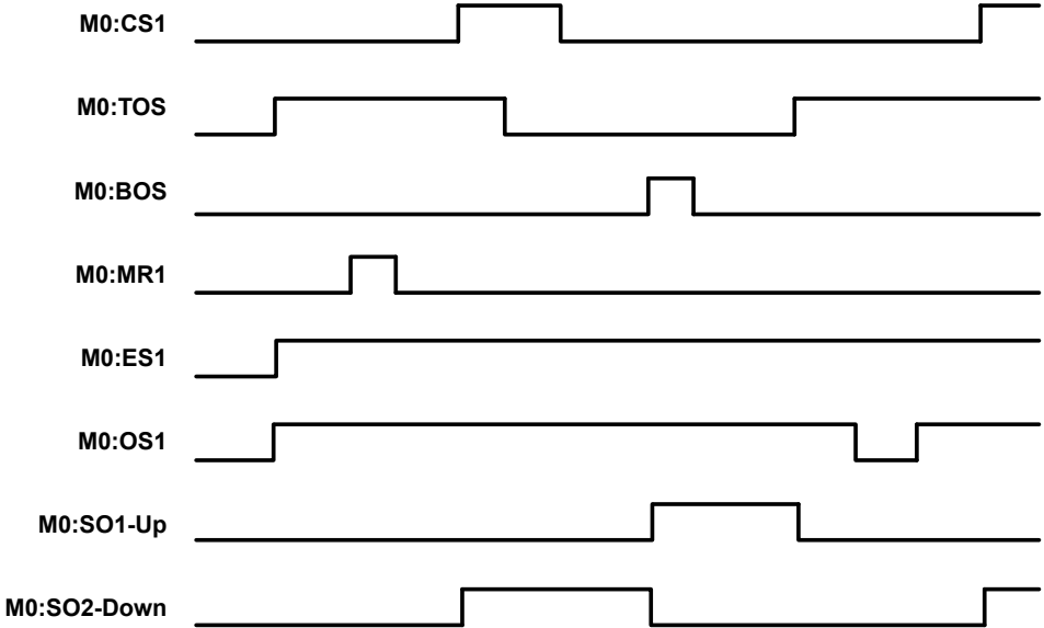
Figure 146. Press Control—Timing Diagram, Single Actuator Control
