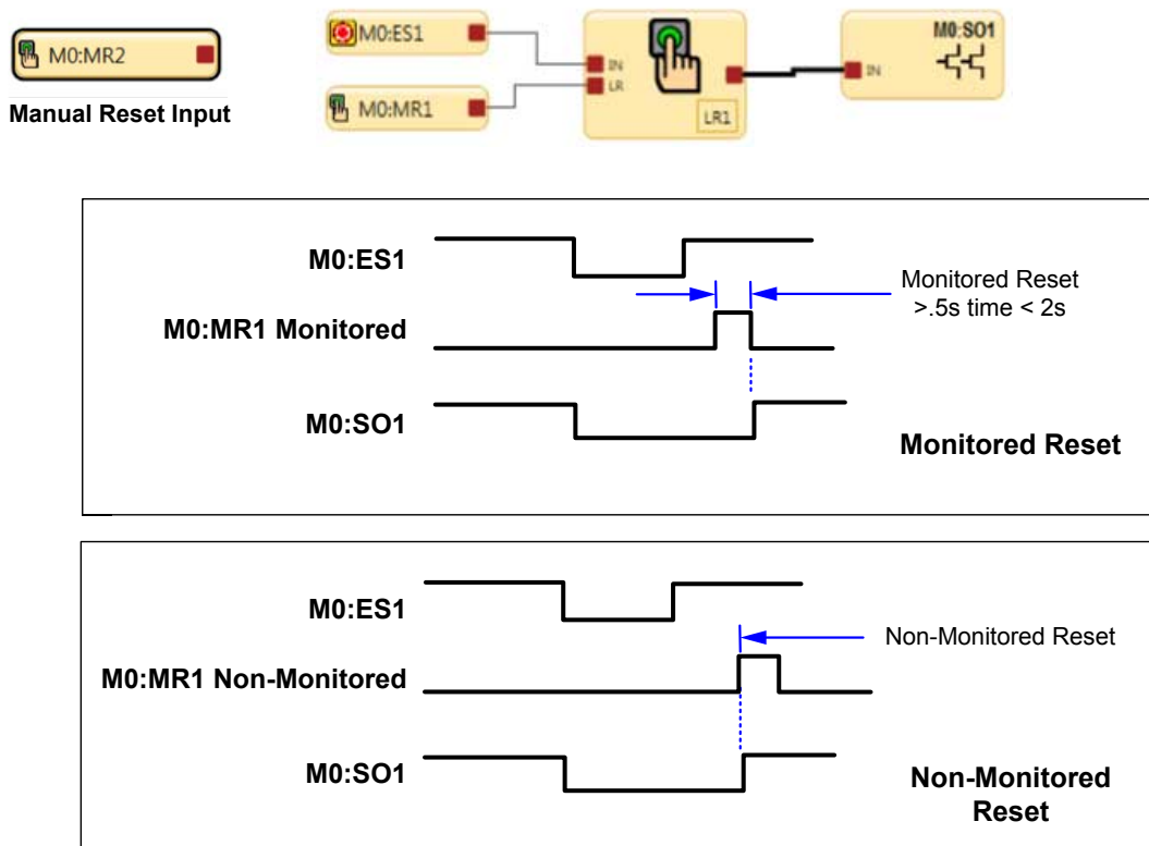
Figure 124. Timing Diagram—Latch Reset Block, Monitored/Non-Monitored Reset
