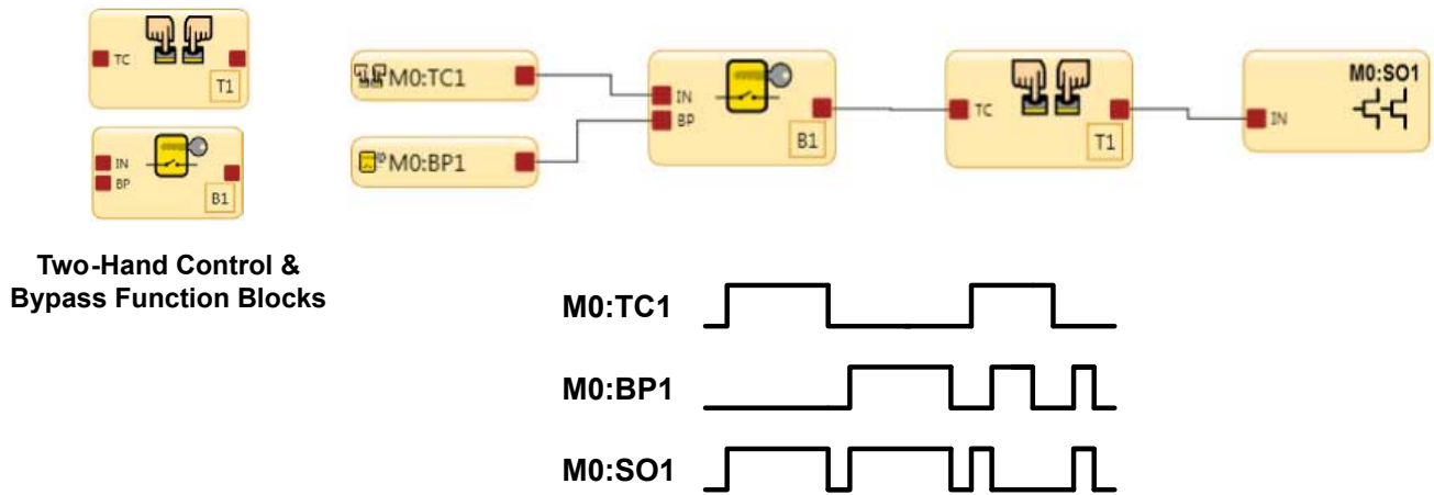
Figure 152. Timing Diagram—Two-Hand Control Block and Bypass Blocks with One (1) Two-Hand Control Input
