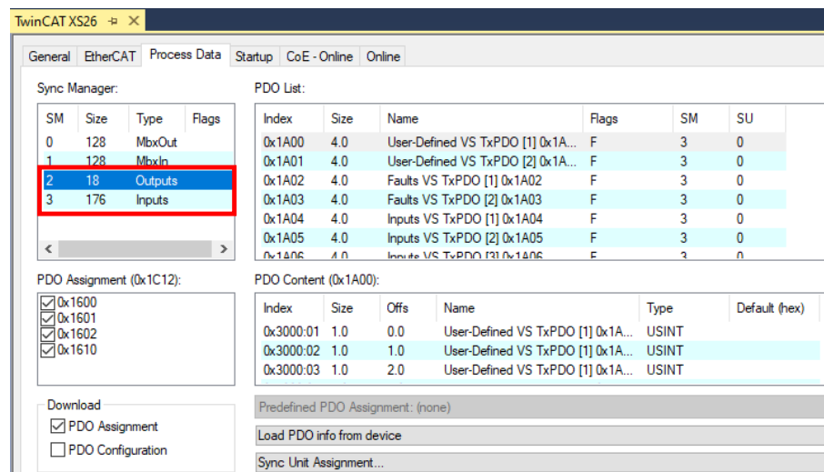
Figure 283. Output and Inputs in Sync Manager
