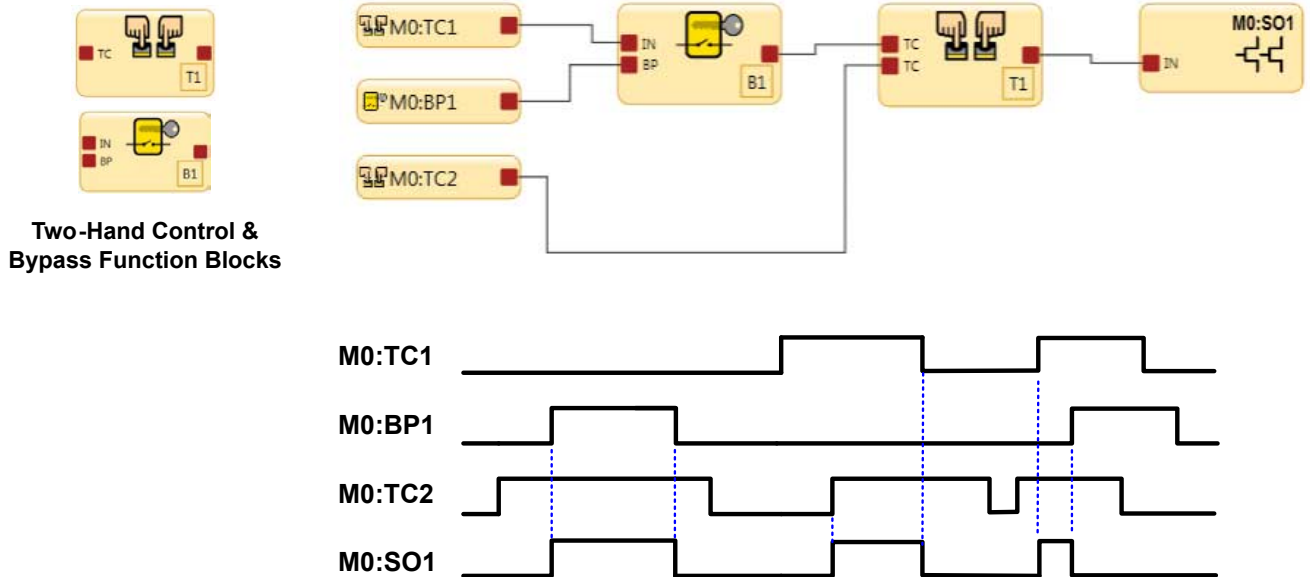
Figure 153. Timing Diagram—Two-Hand Control Block and Bypass Blocks with Two (2) Two-Hand Control Inputs
