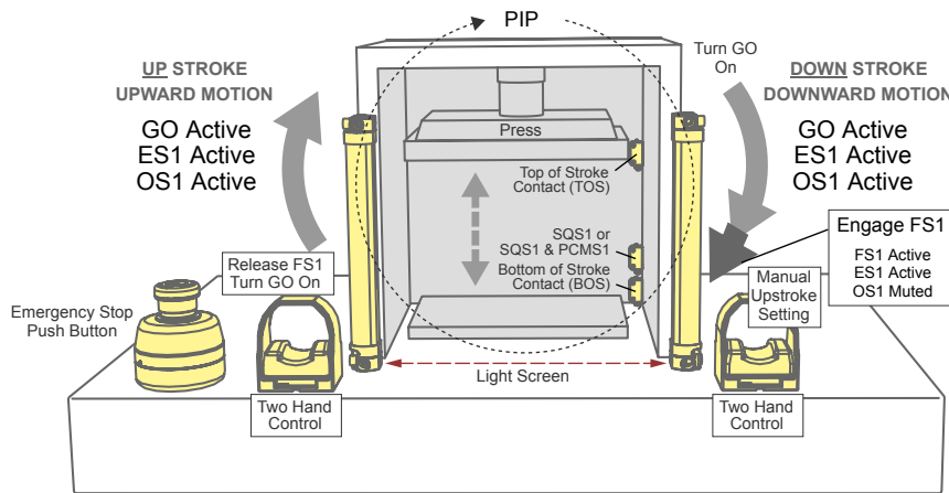
Figure 71. Full Feature Sample Press Control Configuration
