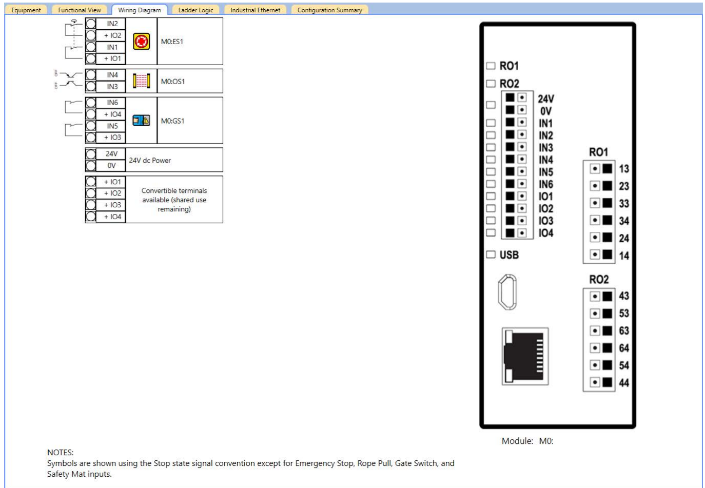
Figure 294. Wiring Diagram tab with an E-stop button, optical sensor, and gate switch
