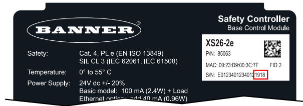
Figure 171. Serial Number
