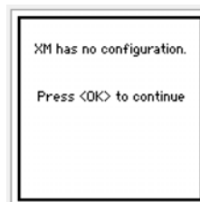
Figure 303. Blank SC-XM2/3
