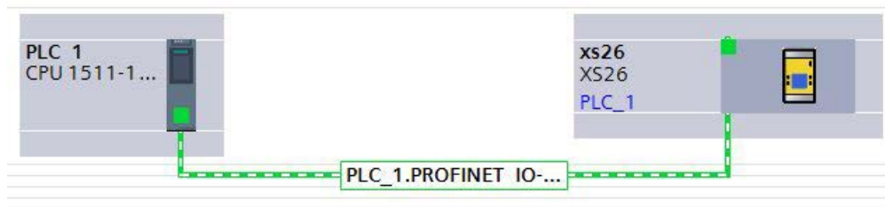
Figure 268. Network View
