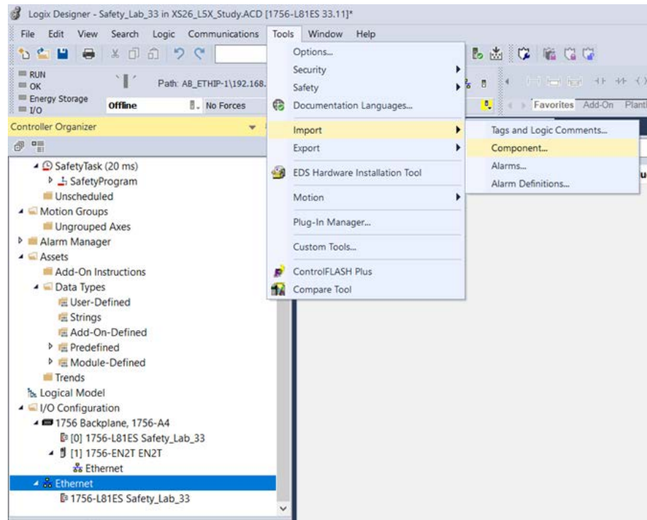
Figure 165. Studio 5000
