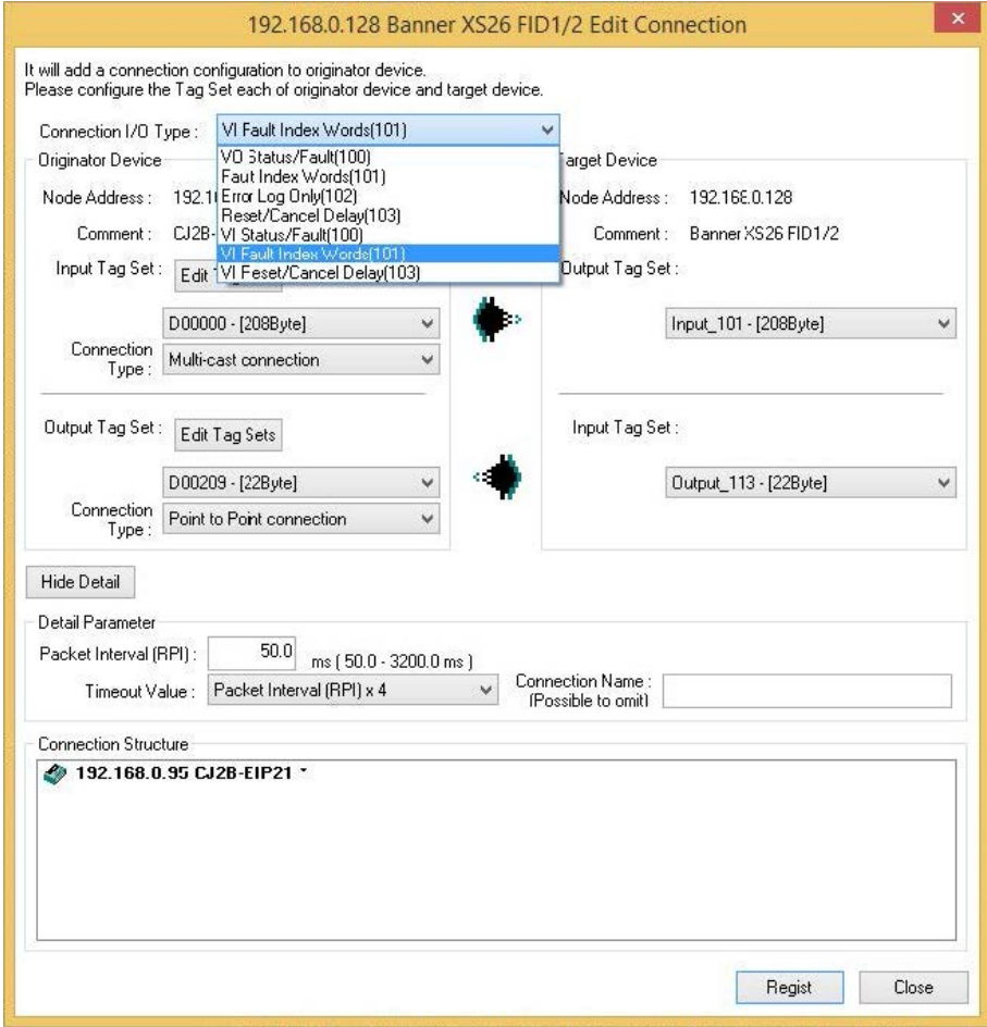
Figure 235. Edit Connections
