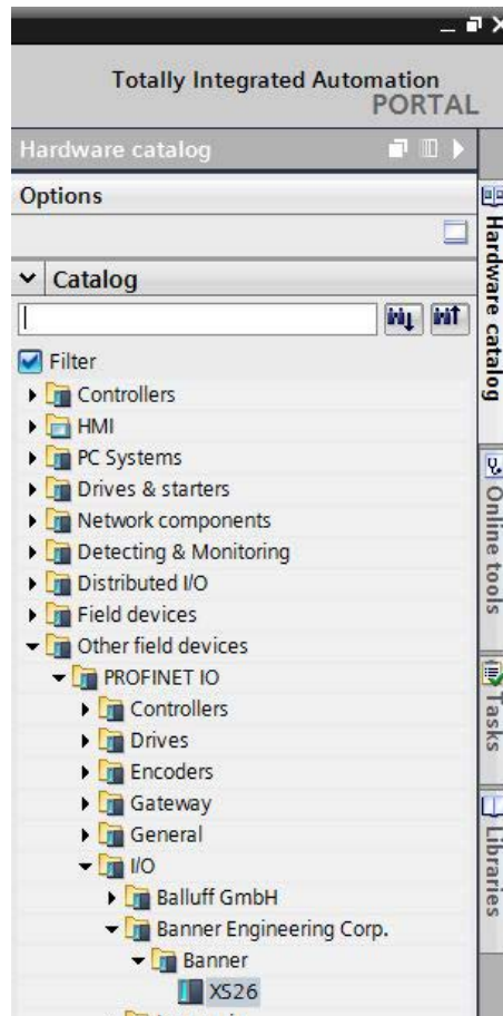
Figure 258. Hardware Catalog
