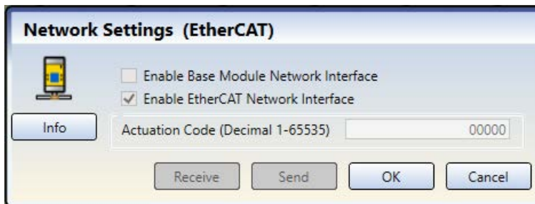
Figure 97. Network Settings—EtherCAT
