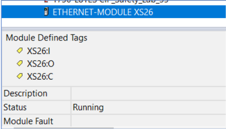
Figure 167. Run Mode
