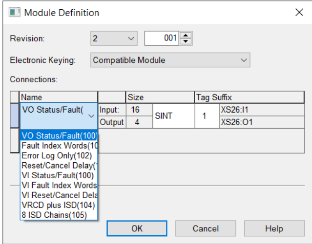
Figure 181. Module Definition
