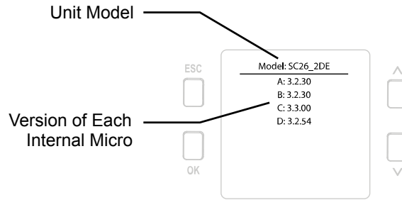
Figure 159. Onboard Interface—Model #
