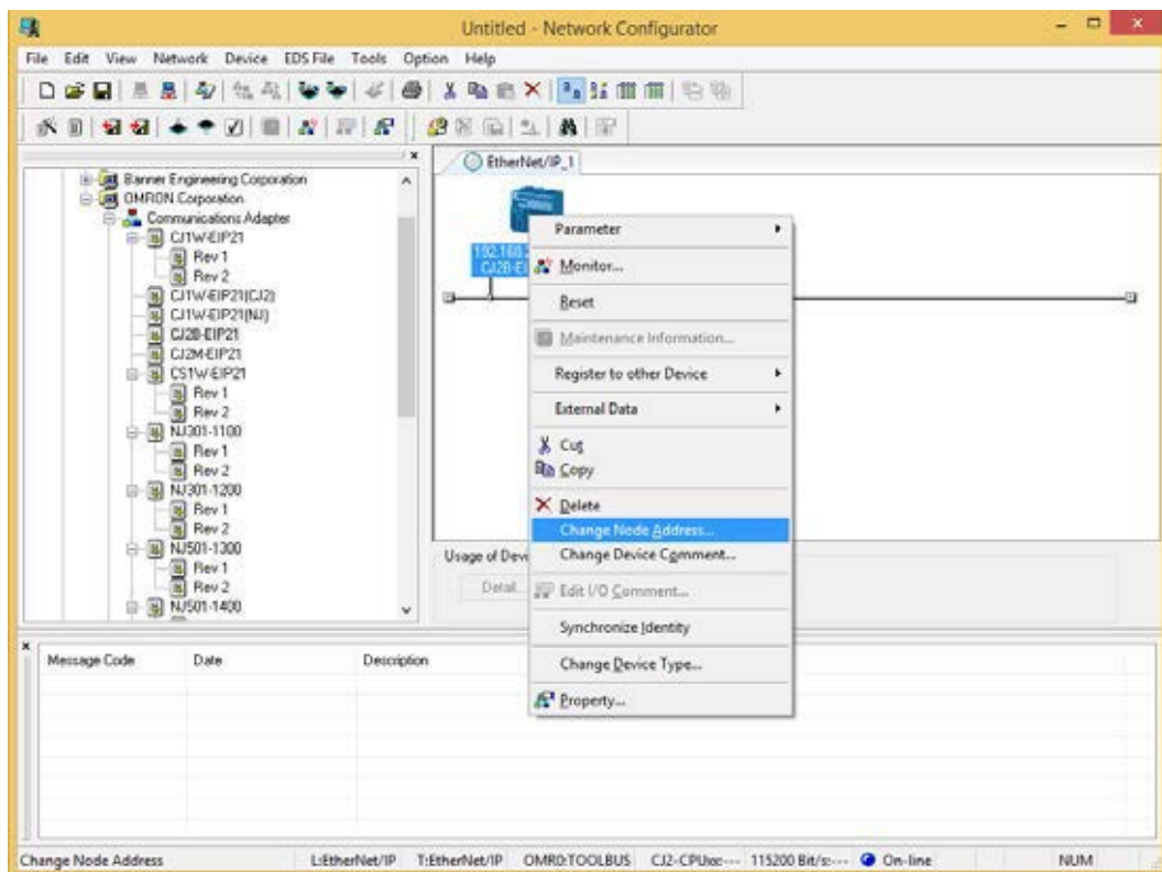
Figure 221. Right-Click Menu
