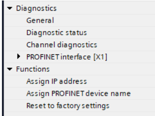
Figure 272. Online & Diagnostics
