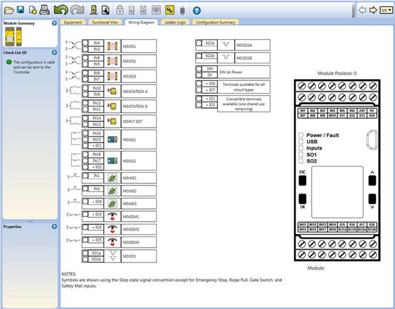
Figure 84. Wiring Diagram Tab—XS26
