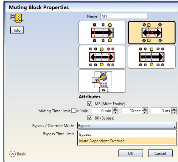
Figure 130. Mute-Dependent Override
