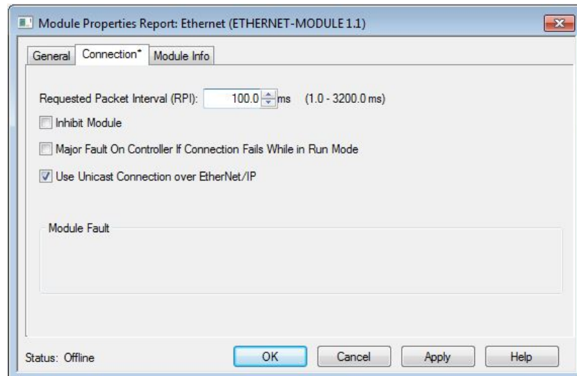
Figure 201. Connection Parameters
