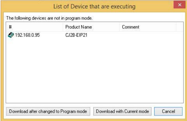
Figure 238. Download Options
