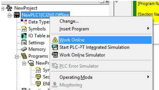
Figure 244. Work Online
