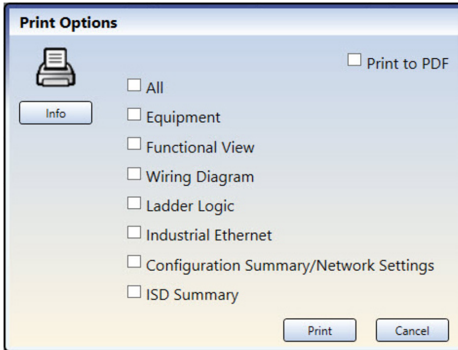
Figure 99. Print Options
