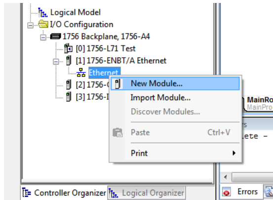
Figure 178. New Module
