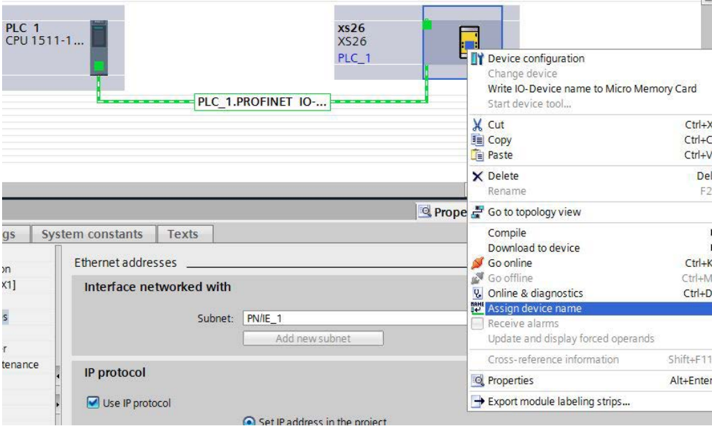
Figure 277. Ethernet Addresses
