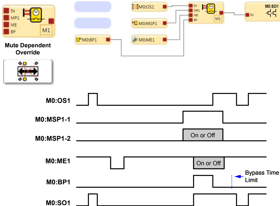
Figure 130. Mute-Dependent Override
