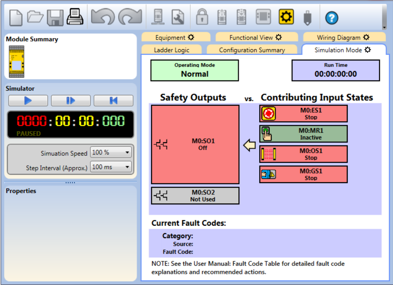
Figure 108. Simulation Mode
