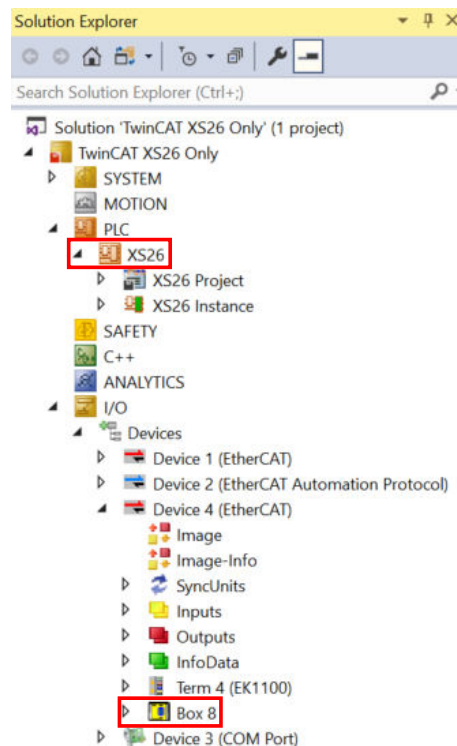
Figure 280. Solution Explorer
