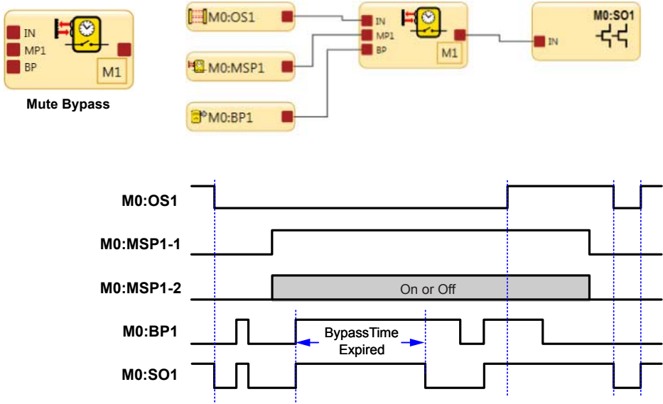
Figure 131. Mute Bypass
