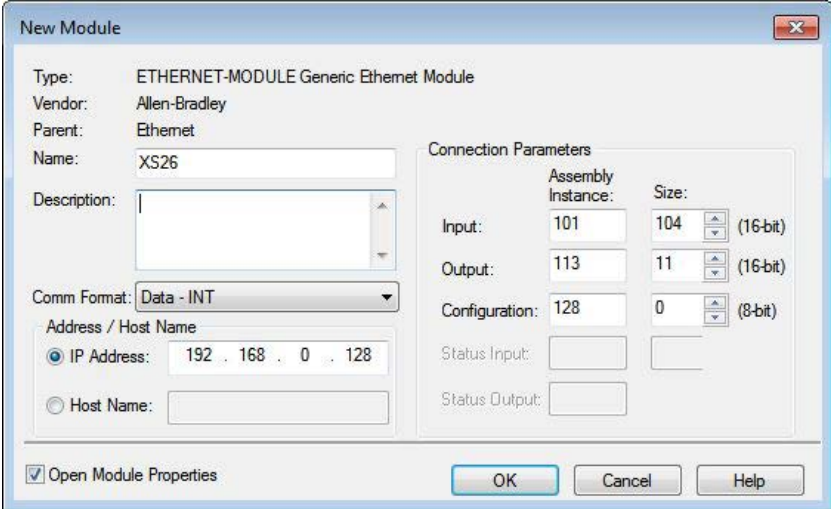
Figure 198. PLC Input Assembly 103 (0x67), size 35 words (VI Reset/Cancel Delay)
