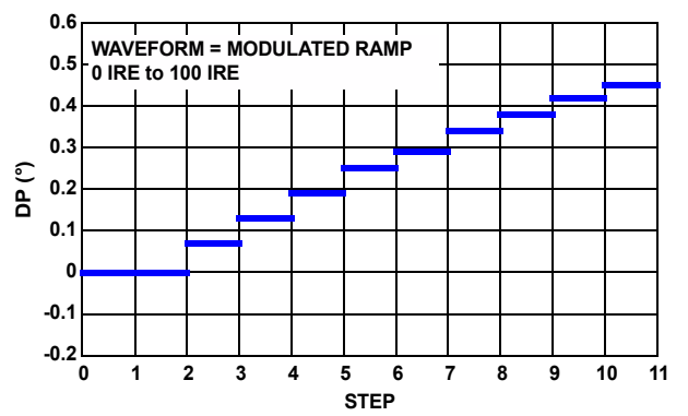
FIGURE 12. DIFFERENTIAL PHASE
