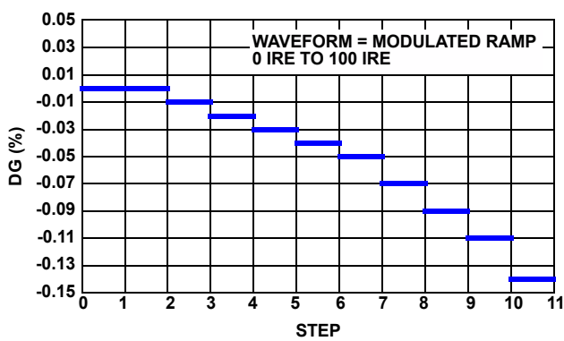
FIGURE 11. DIFFERENTIAL GAIN
