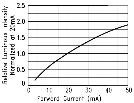
Fig.4 RELATIVE LUMINOUS INTENSITY VS. FORWARD CURRENT 0° 10° 20°
