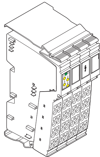
Figure 1 IB IL 24/230 DOR 4/W-PC terminal with connectors
