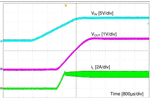
Figure 15. DCM Mode
