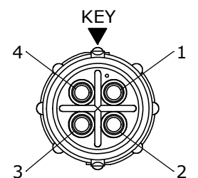
WIRE VIEW W8380-4PG-P-3XX
