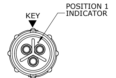
WIRE VIEW W8380-3PG-P-3XX SHOWN
