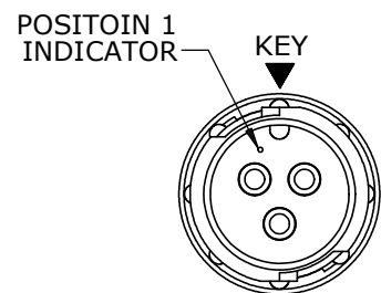
FACE VIEW W8380-3PG-P-3XX SHOWN
