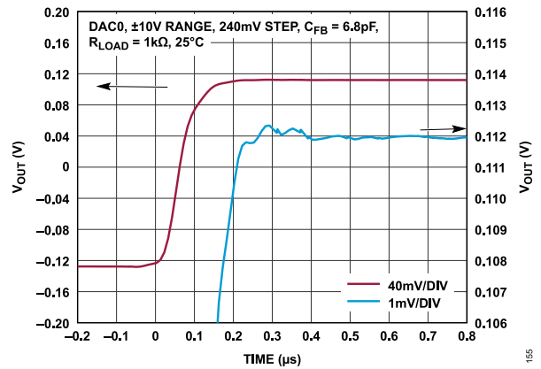
Figure 53. Small Signal Settling Time, -10 V to +10 V Range
