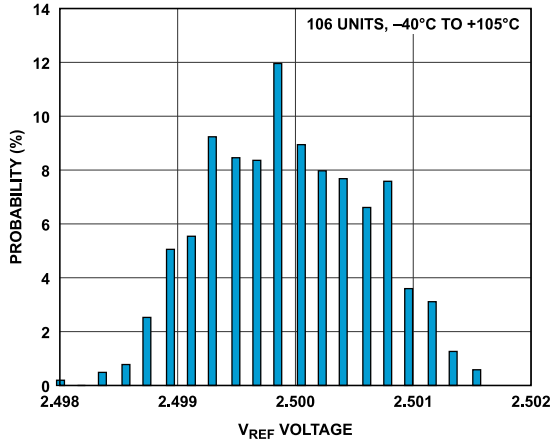
Figure 61. Reference Voltage Spread
