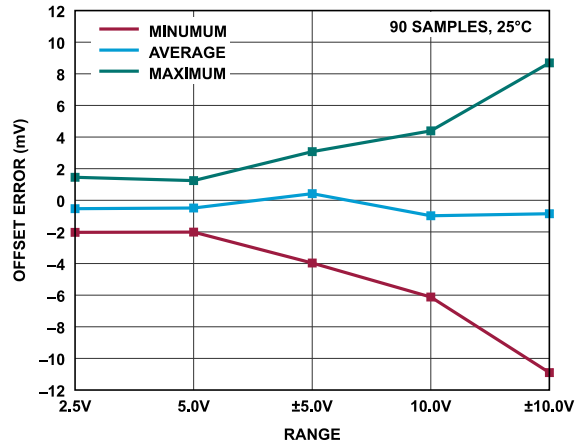
Figure 28. Offset Error vs. Range
