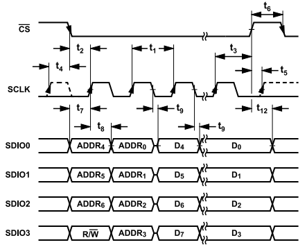
Figure 9. Quad SPI Read Operation with Single Data Rate
