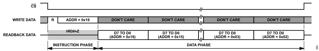
Figure 74. Streaming Mode Register Read with Address Descending
