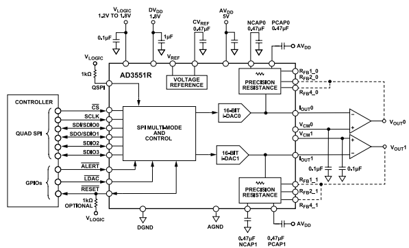
Figure 91. Recommended Application Circuit
