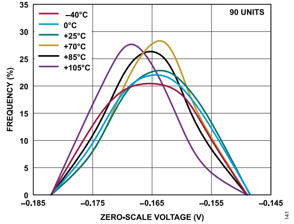
Figure 40. Zero-Scale Voltage Distribution, 0 V to 10 V Range
