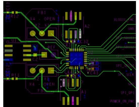
Figure 92. EVAL-AD3552R Component Arrangement and Layout
