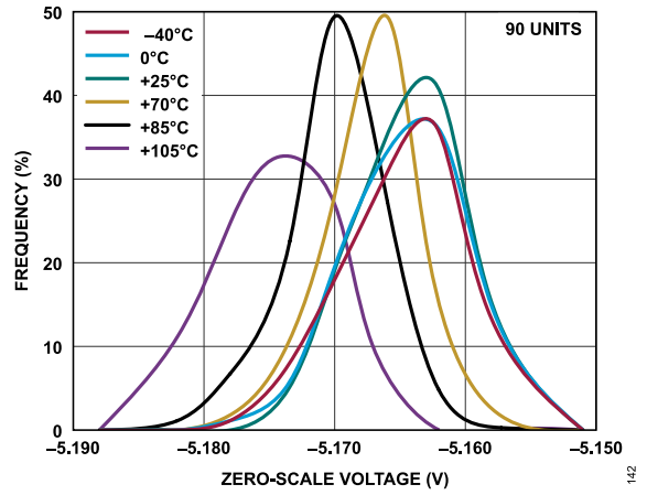
Figure 41. Zero-Scale Voltage Distribution, -5 V to +5 V Range
