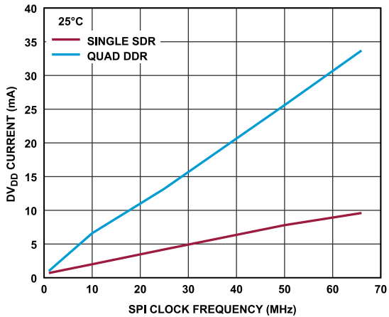
Figure 63. DV_{DD} Current vs. SPI Clock Frequency, SPI Mode
