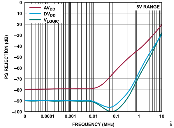
Figure 58. AC PSRR
