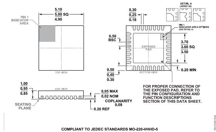
COMPLIANT TO JEDEC STANDARDS MO-220-VHHD-5 Figure 93. 32-Lead Lead Frame Chip Package [LFCSP] 5 mm × 5 mm Body and 0.95 mm Package Height (CP-32-30) Dimensions shown in millimeters
