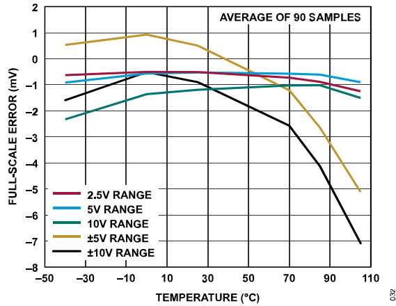
Figure 31. Full-Scale Error vs. Temperature
