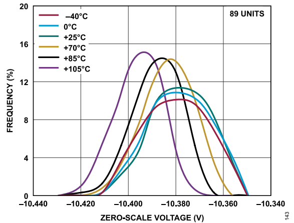
Figure 42. Zero-Scale Voltage Distribution, -10 V to +10 V Range
