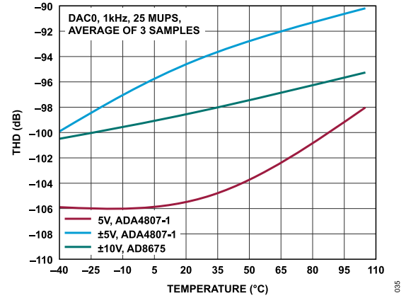
Figure 34. THD vs. Temperature
