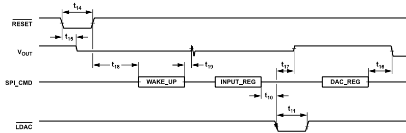
Figure 11. Start-Up Sequence Timing
