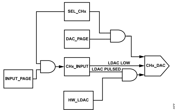
Figure 88. DAC Data Flow Between Registers
