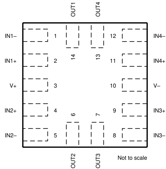
Not to scale Figure 6-11. OPA4310 RUC Package, 14-Pin X2QFN (Top View)
