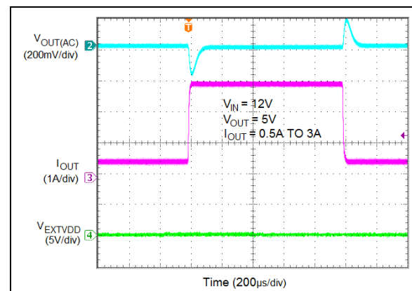
FIGURE 4-4: V_{OUT} Load Transient with EXTVDD Connected to Ground.
