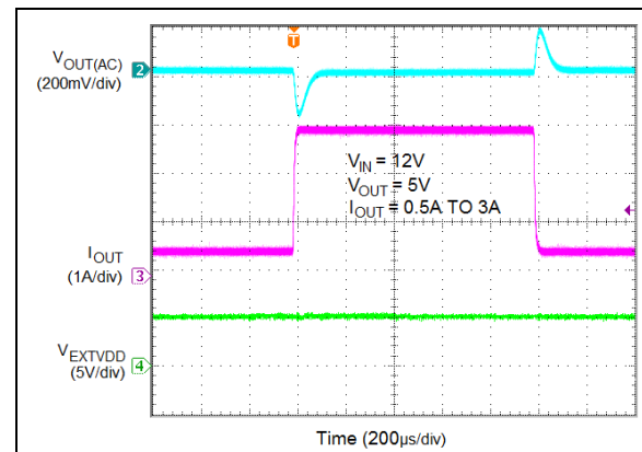
FIGURE 4-3: V_{OUT} Load Transient with EXTVDD Connected to V_{OUT} .
