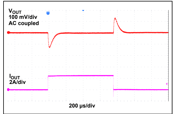
FIGURE 2-40: Load Transient Response (0 to 2.5A).
