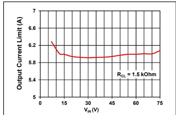
FIGURE 2-23: Output Current Limit vs. Input Voltage.
