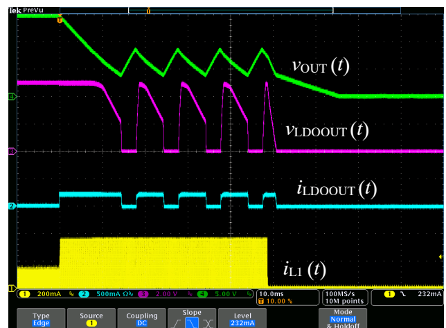
Figure 34. LDO Over-current Protection – Over-loaded LDO Rail, I_{OUT} = 30\text{mA} , I_{LDOOUT} = 30\text{mA} to 200\text{mA} , V_{IN} = 230\text{V}
