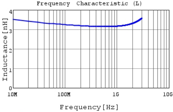
LQG15WH3N2S02 L
