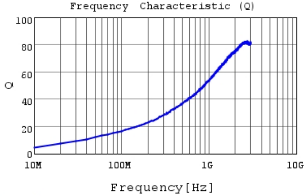
LQG15WH3N2S02 Q
