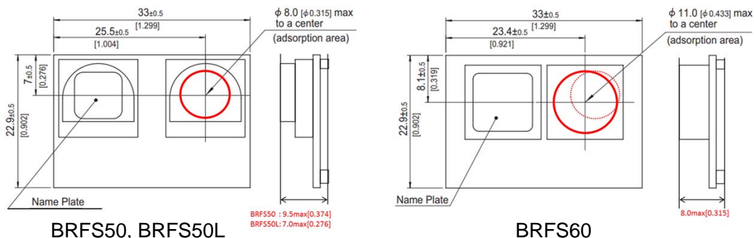
Figure 2.1 Differences of Dimensions between BRFS50, BRFS50L and BRFS60
