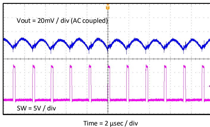
Figure 4-8. TPS56C230EVM Output Ripple, 12-A Load
