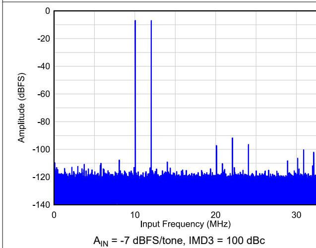
Figure 6-45. Two Tone FFT at F_{IN} = 10, 12 MHz
