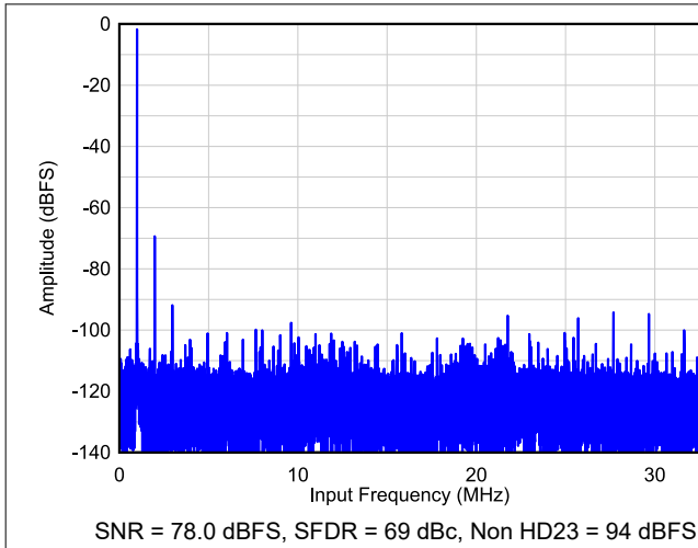
Figure 6-43. Single Tone FFT at F_{IN} = 64 MHz
