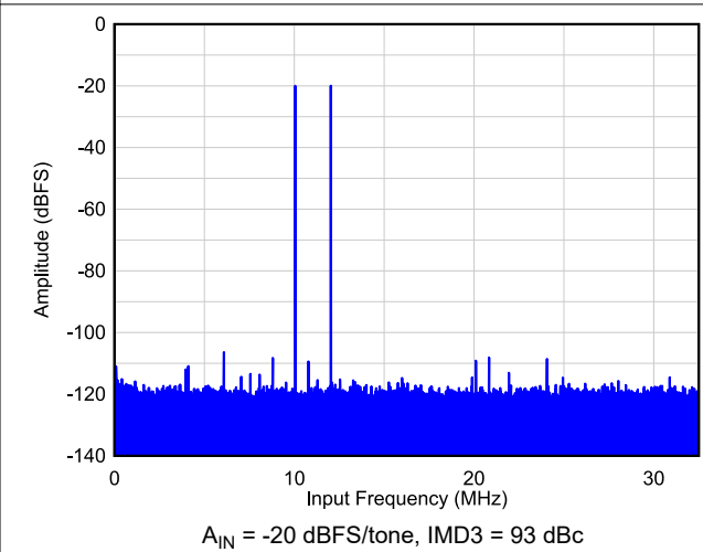
Figure 6-46. Two Tone FFT at F_{IN} = 10, 12 MHz
