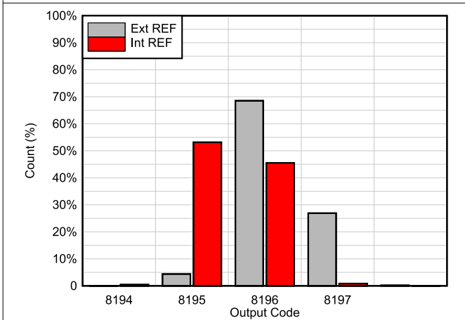
Figure 6-34. DC Histogram
