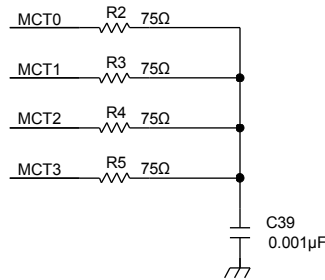
Figure 38. Magnetics
