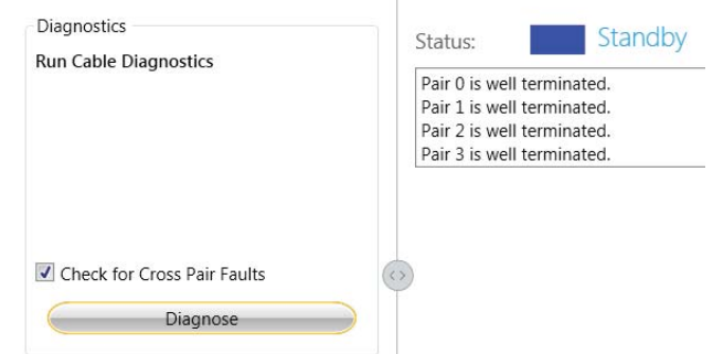
Figure 27. Cable Diagnostics Configuration when Link is Disabled with Cable Connected to Remote PHY
