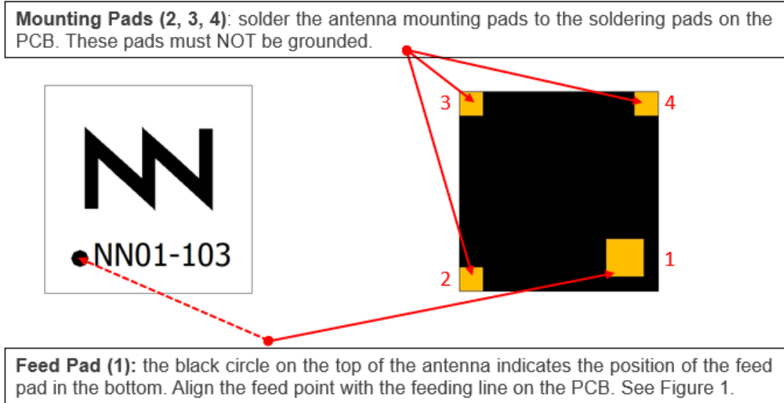
Figure 2 – Pads of the Geofind ™ chip antenna.
