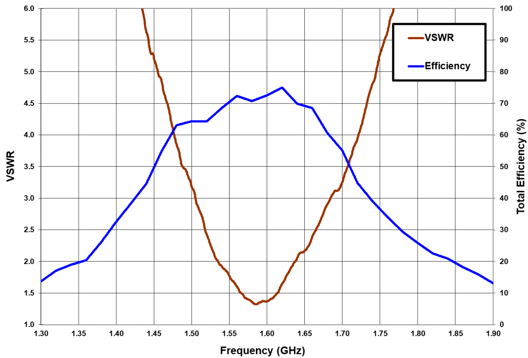
Figure 3 – VSWR and Efficiency (%) vs. Frequency (GHz).
