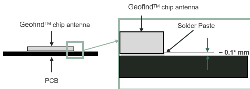
Figure 3 – Soldering Details.
