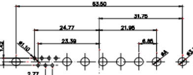
13W6 Female
