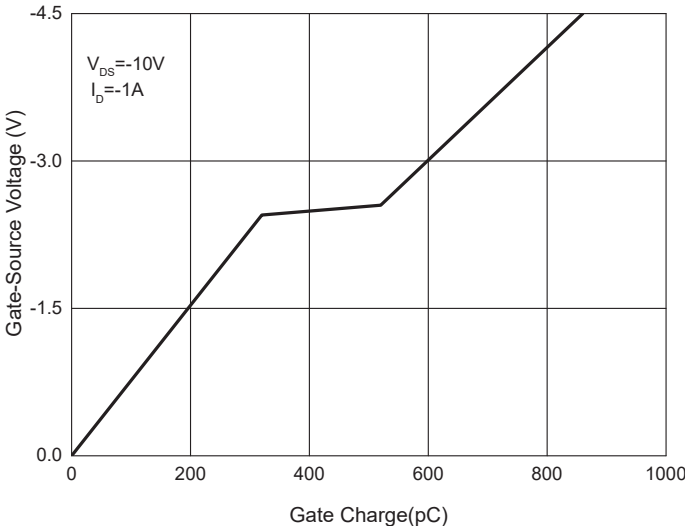
Fig. 8 - Gate Charge
